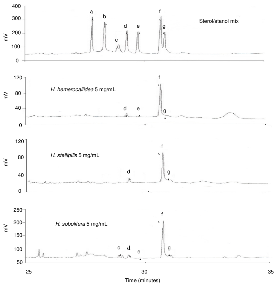
Figure 2. GC chromatograms of standards and chloroform Hypoxis extracts: (a) cholesterol, (b) fucosterol, (c) desmosterol/ergosterol, (d) campsterol, (e) stigmasterol, (f) β-sitosterol and (g) stigmasterol.
