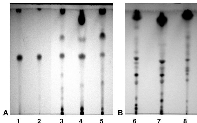
Figure 1. TLC plate of the (A) sterols and (B) sterolins found in chloroform Hypoxis spp. extracts (1) \beta -sitosterol, (2) stigmasterol, (3/6) H. hemerocallidea , (4/7) H. sobolifera and (5/8) H. stellipilis .
