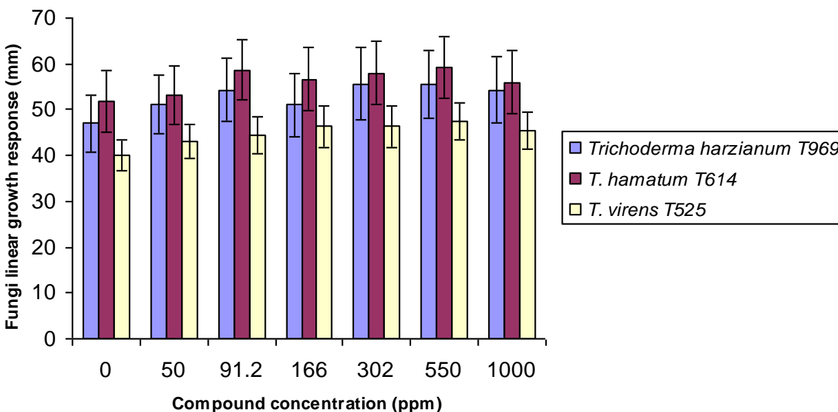
Figure 2. Radial growth response of T. harzianum T969, T. hamatum T614 and T. virens T525 on potato dextrose agar (PDA) medium amended with 0, 50, 91.2, 166, 302, 550 and 1000 mg/l (ppm) of \text{MgSO}_4 \cdot 7\text{H}_2\text{O} . Bars represent standard errors (SE).
