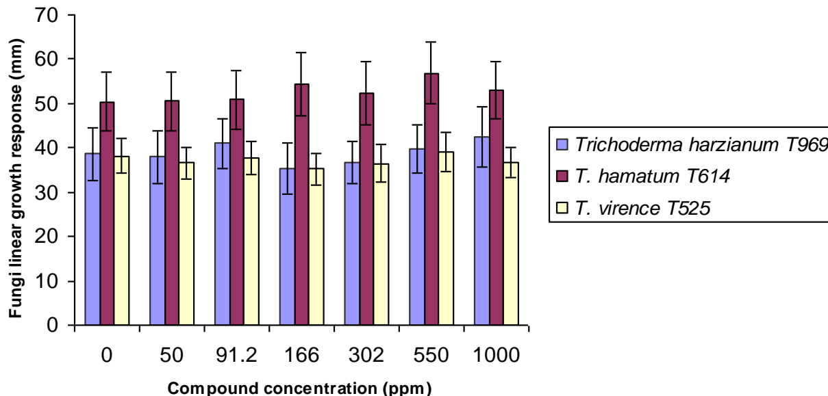
Figure 1. Radial growth response of T. harzianum T969, T. hamatum T614 and T. virens T525 on potato dextrose agar (PDA) medium amended with 0, 50, 91.2, 166, 302, 550 and 1000 mg/l (ppm) of (\text{NH}_4)_2\text{SO}_4 . Bars represent standard errors (SE).
