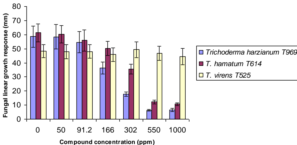
Figure 7. Radial growth response of T. harzianum T969, T. hamatum T614 and T. virens T525 on potato dextrose agar (PDA) medium amended with 0, 50, 91.2, 166, 302, 550 and 1000 mg/l (ppm) of \text{MnSO}_4 \cdot \text{H}_2\text{O} . Bars represent standard errors (SE).
