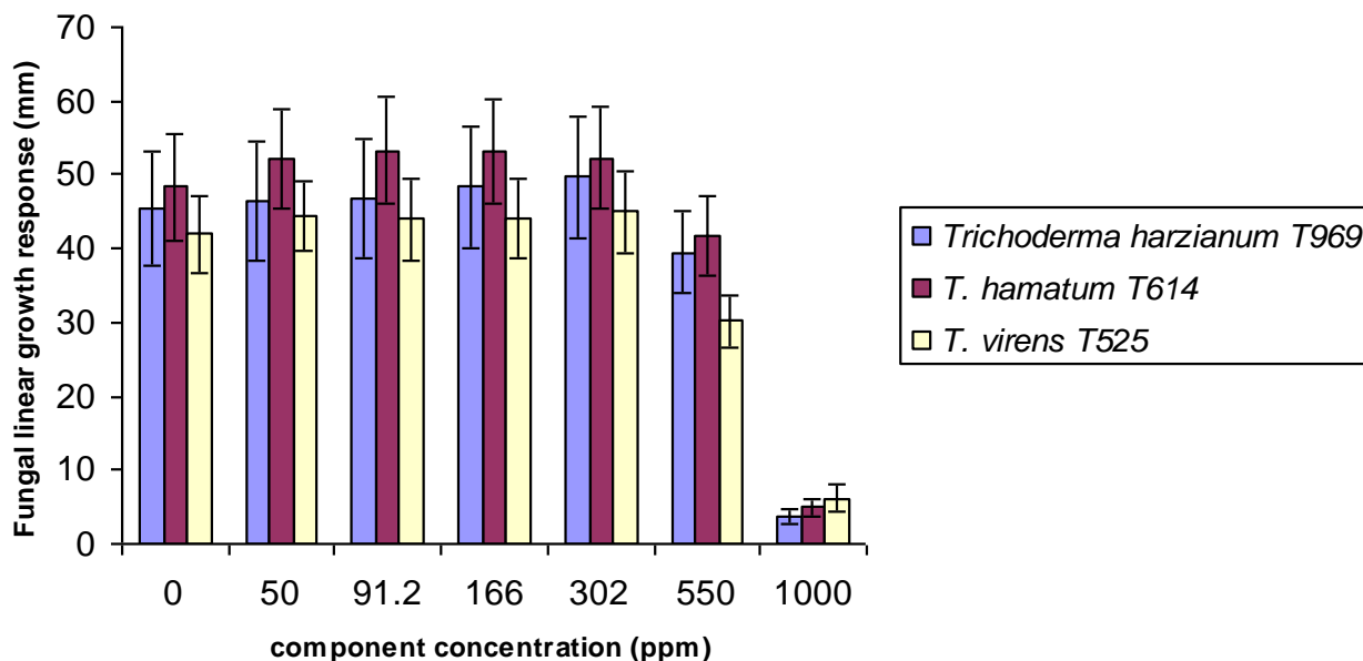
Figure 6. Radial growth response of T. harzianum T969, T. hamatum T614 and T. virens T525 on potato dextrose agar (PDA) medium amended with 0, 50, 91.2, 166, 302, 550 and 1000 mg/l (ppm) of \text{FeSO}_4 \cdot 7\text{H}_2\text{O} . Bars represent standard errors (SE).
