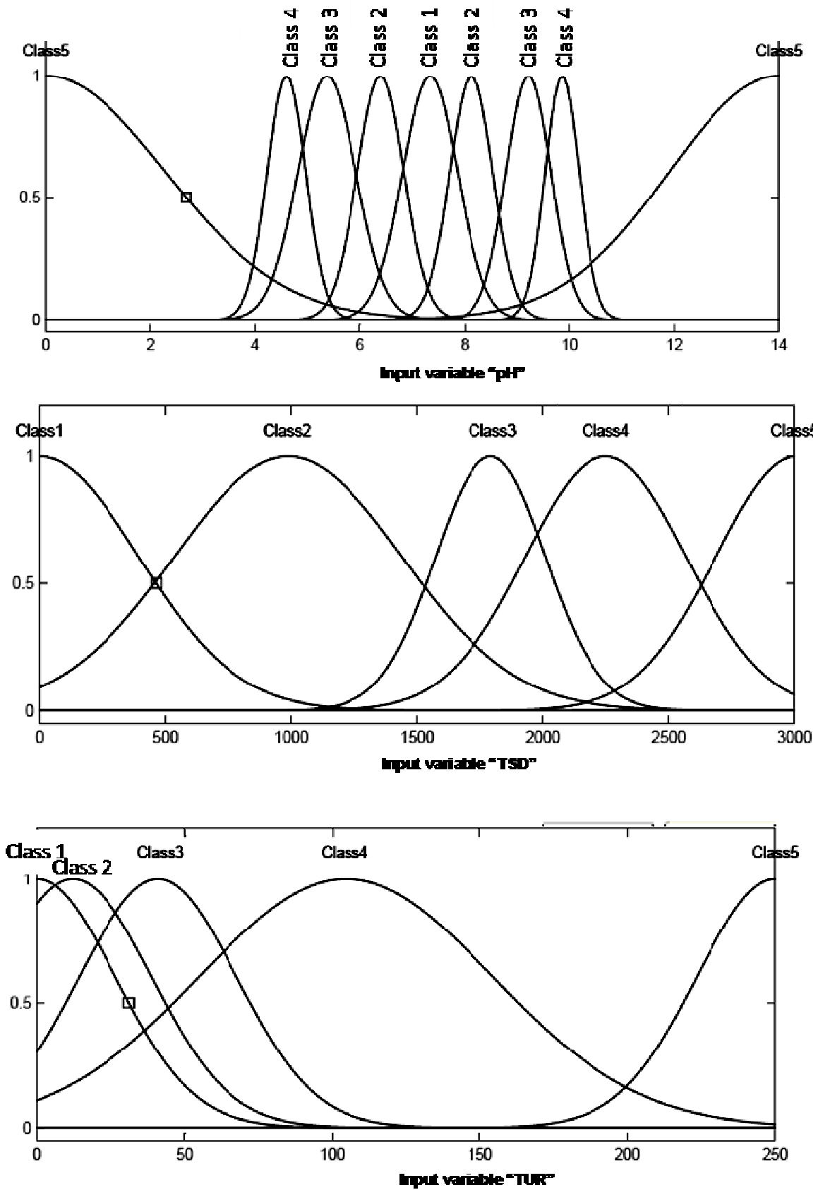
Figure 1. Membership functions defined for water quality classification.
