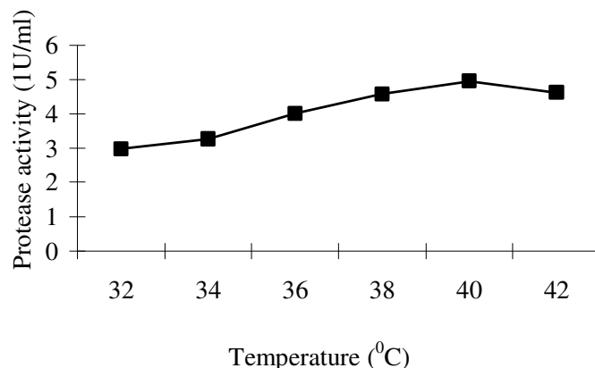
Figure 3. Effect of Temperature on protease activity of strain PS-18A.
