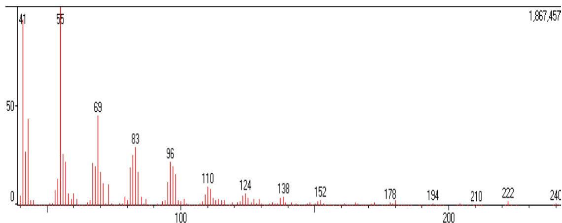
Figure 1. The mass spectrum of cyclopentadecanolide sample at retain time t= 11.703 min in gas chromatography.
