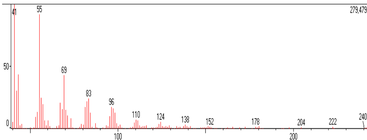
Figure 2. The mass spectrum of product at retain time t= 11.703 min in gas chromatography.
