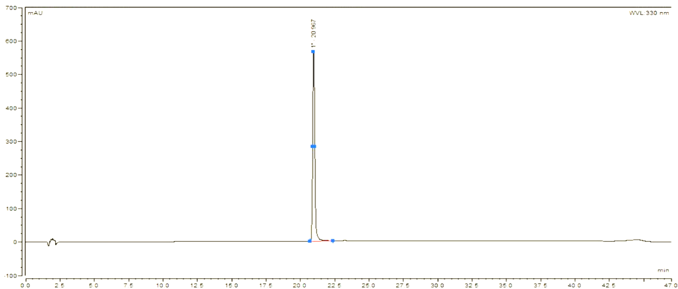
Figure 1. Chromatogram of luteolin standard.
