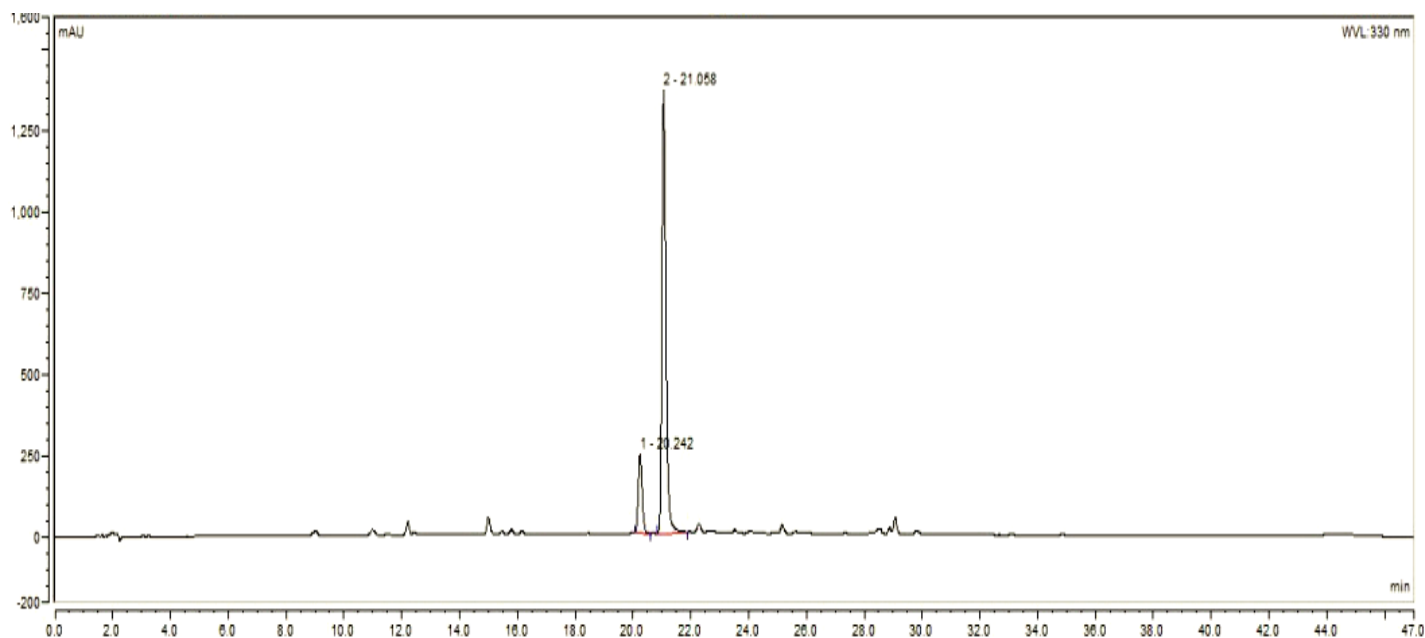
Figure 2. Chromatogram of luteolin content in Mikwang peanut shell.
