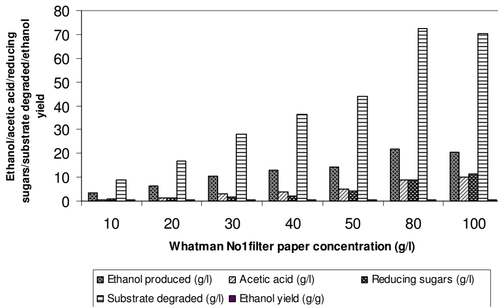
Figure 4. Coculture fermentation of high concentration of Whatman No 1 filter paper to ethanol by C. thermocellum CT2 with C. thermosaccharolyticum HG8.
