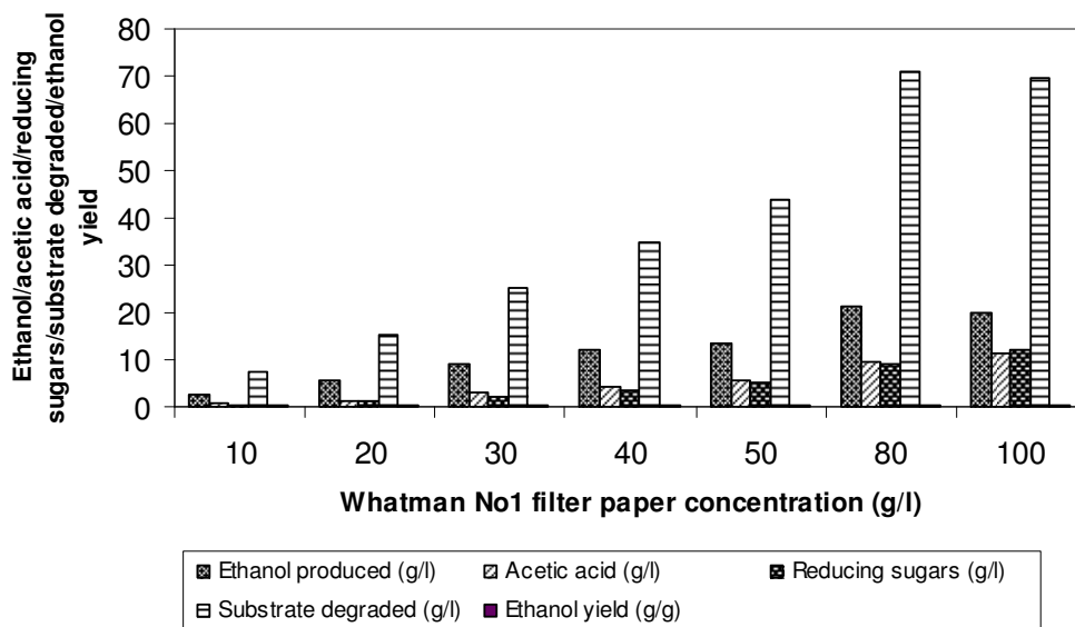
Figure 5. Coculture fermentation of high concentration of Whatman No1 filter paper materials to ethanol by C. thermocellum CT2 with C. ethanolicus ATCC 31937.
