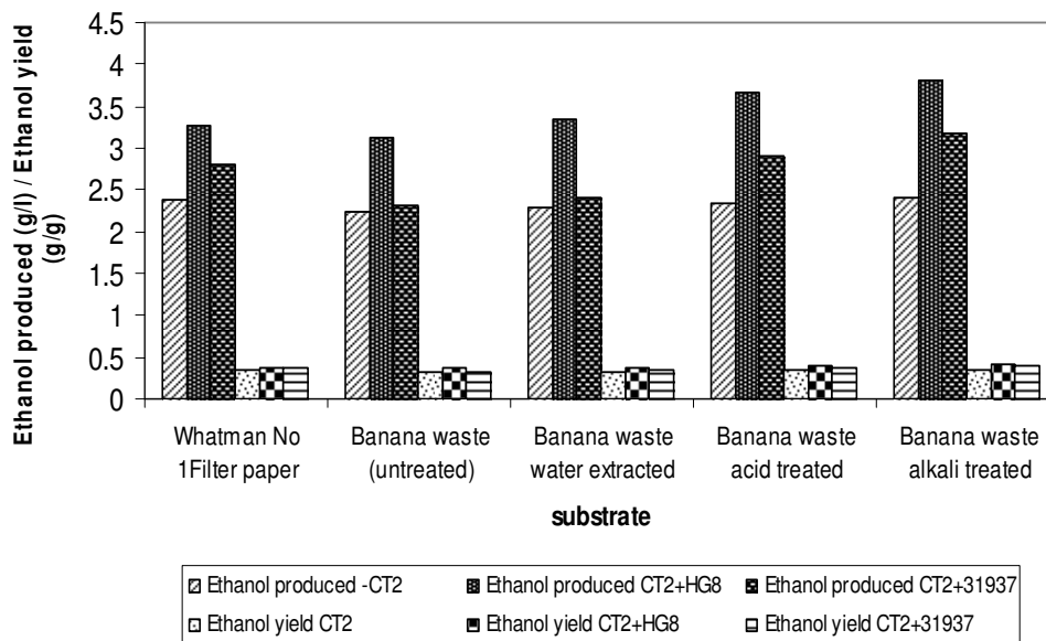
Figure 2. Ethanol produced and ethanol yields in mono and coculture fermentations of banana leaves by C. thermocellum CT2 with HG8 and ATCC 31937.
