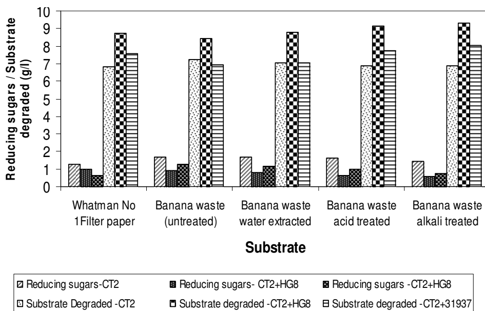
Figure 3. Substrate degraded and reducing sugars formed in mono and coculture fermentations of banana leaves by C. thermocellum CT2 with HG8 and ATCC 31937.
