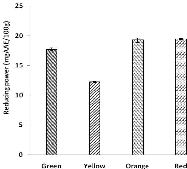
Figure 1. Reducing power of OFI ethanol extracts.
