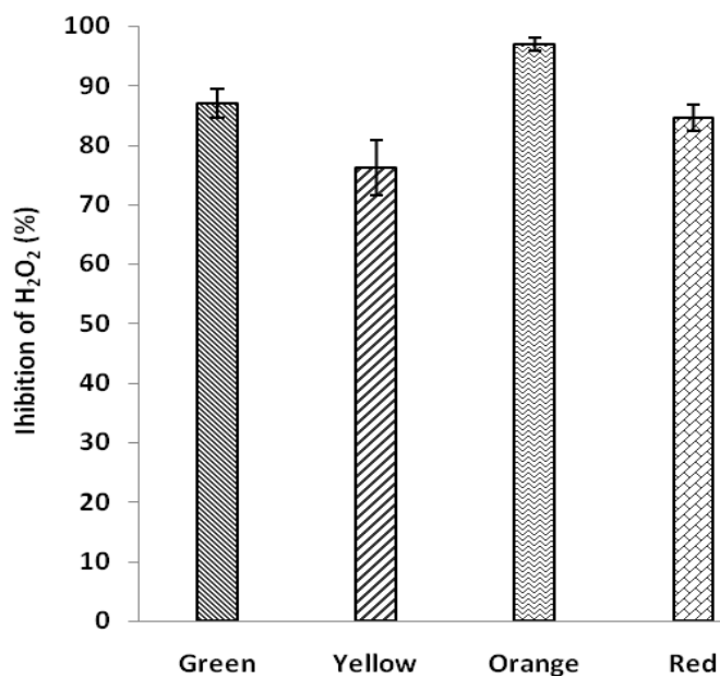
Figure 3. Scavenging activity of OFI ethanol extracts on hydrogen peroxide.
