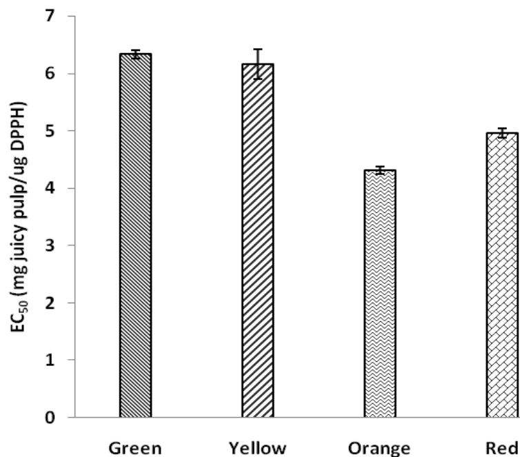
Figure 2. Scavenging activities of OFI ethanol extracts on the DPPH radical (EC 50 ).
