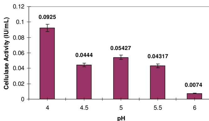
Figure 3. Effect of pH on Aspergillus niger cellulase activity using saw dust as substrate.
