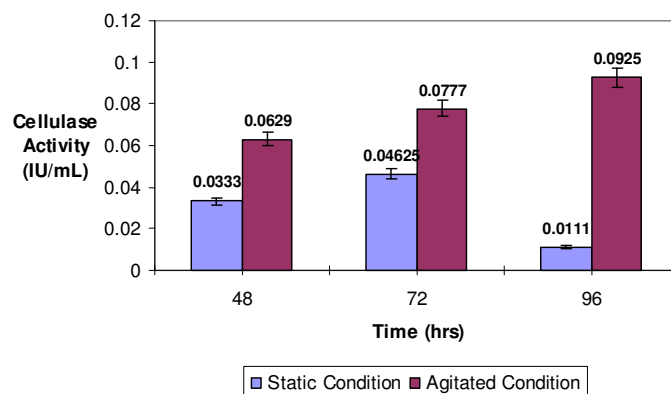
Figure 9. Effect of static and agitated conditions on Aspergillus niger cellulase activity using saw dust as substrate.
