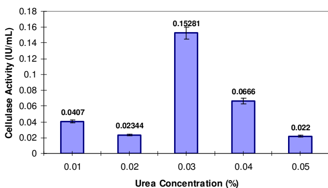
Figure 8. Effect of urea on Aspergillus niger cellulase activity using saw dust as substrate.
