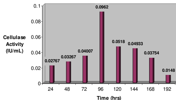
Figure 5. Effect of time duration on Aspergillus niger cellulase activity using saw dust as substrate.
