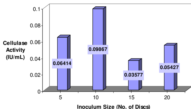
Figure 4. Effect of inoculum size on Aspergillus niger cellulase activity using saw dust as substrate.
