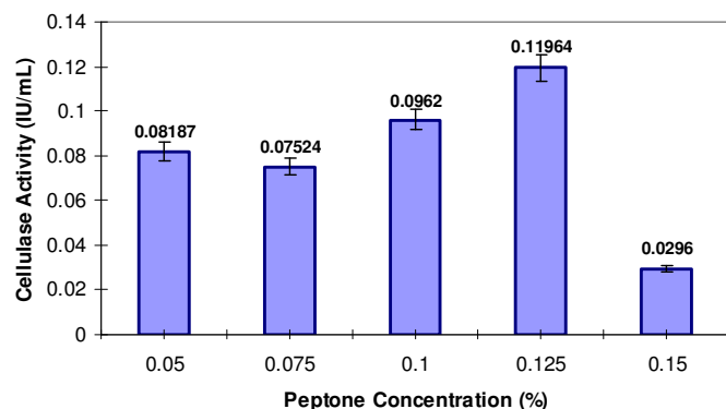
Figure 6. Effect of peptone on Aspergillus niger cellulase activity using saw dust as substrate.
