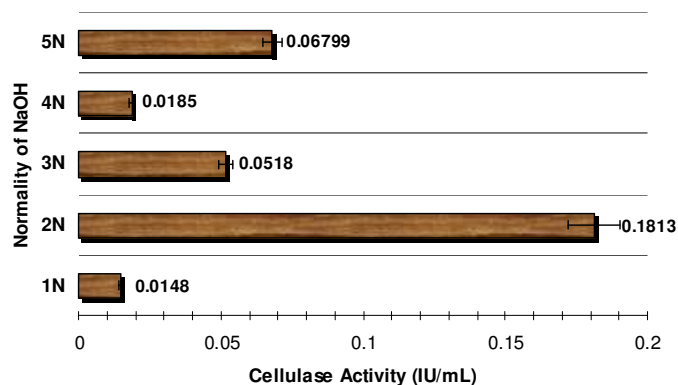
Figure 1. Effect of NaOH pretreatment on Aspergillus niger cellulase activity using saw dust as substrate.
