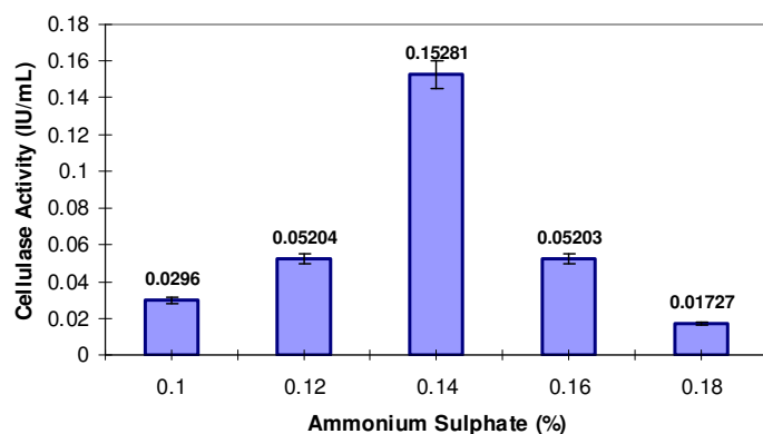
Figure 7. Effect of (\text{NH}_4)_2\text{SO}_4 on Aspergillus niger cellulase activity using saw dust as substrate.
