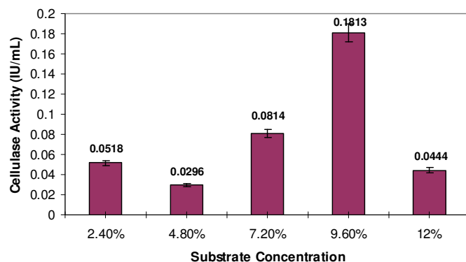
Figure 2. Effect of substrate concentration on Aspergillus niger cellulase activity using saw dust as substrate.
