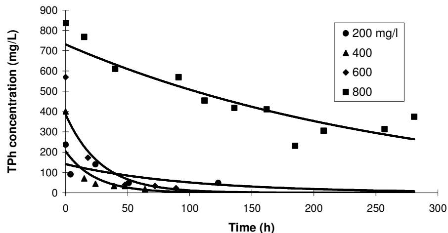
Figure 1. TPH concentration versus degradation time.
