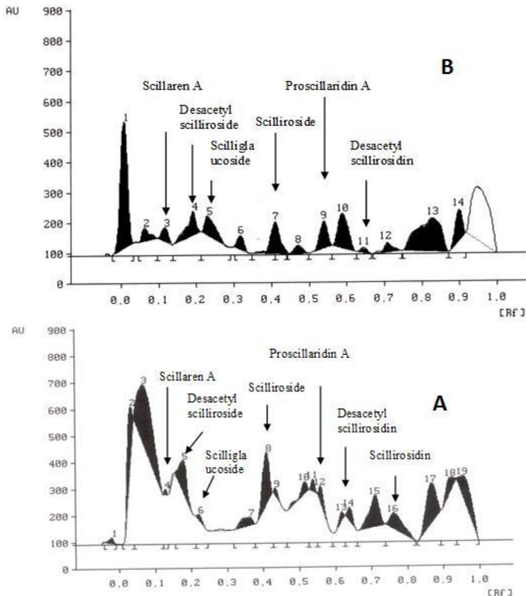
Figure 4. Densitograms showing separation of individual components in (A) Crude extract, (B) Callus extract by reflectance scanning densitometry on HPTLC plates.
