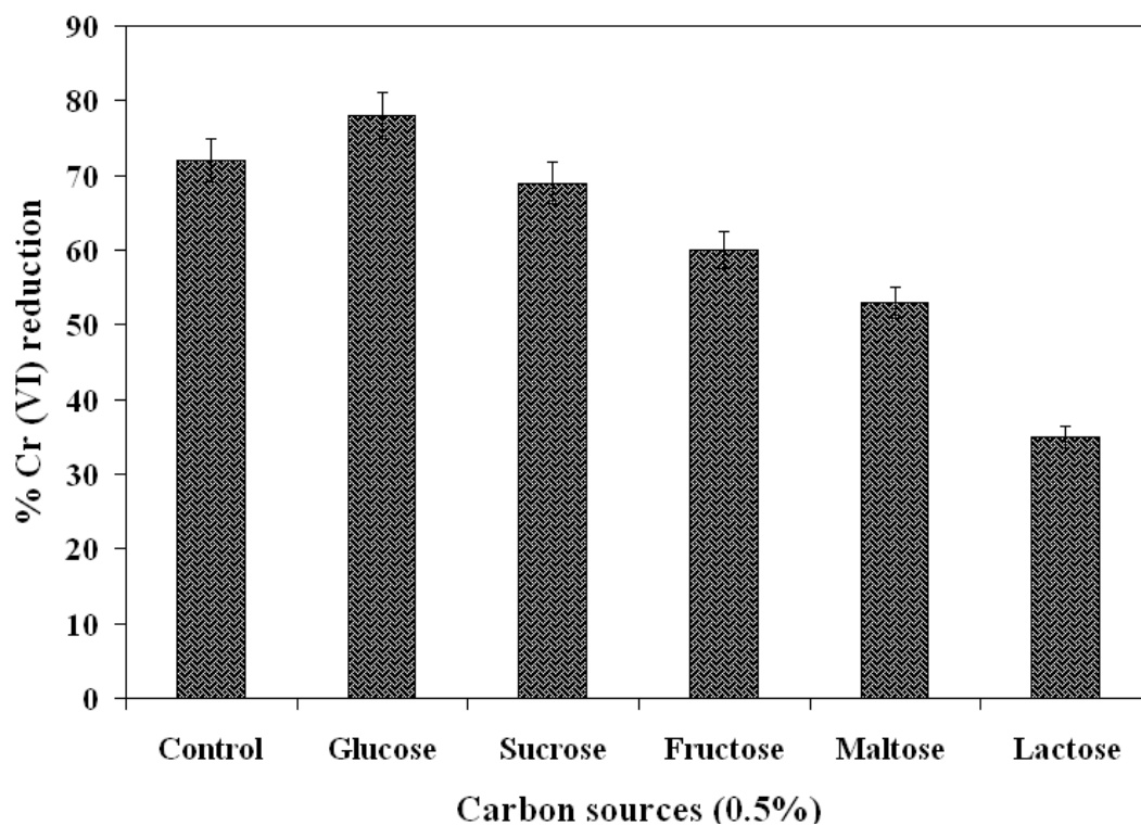
Figure 5. Effect of different carbon sources (0.5%) on Cr (VI) reduction at 1000 \mu\text{g/ml} Cr (VI) concentration. Control does not include any carbon source.
