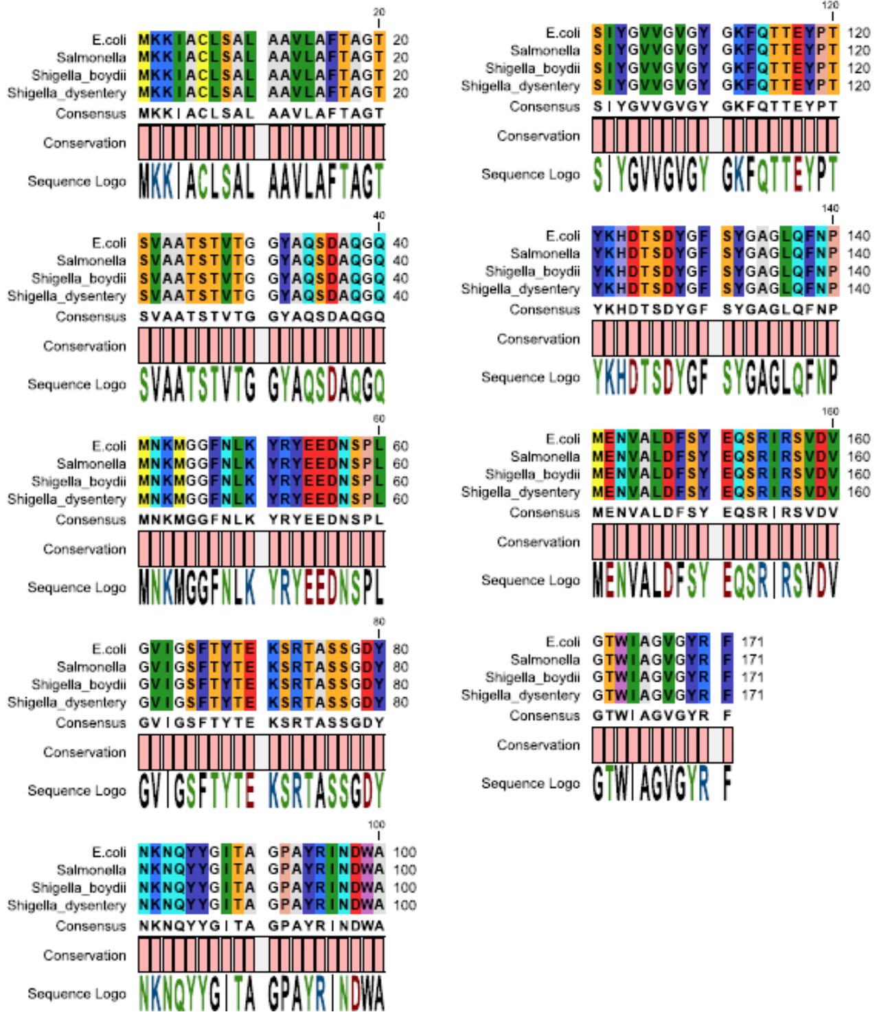
Figure 2. Multiple sequence alignment of common proteins causing diarrheal diseases.
