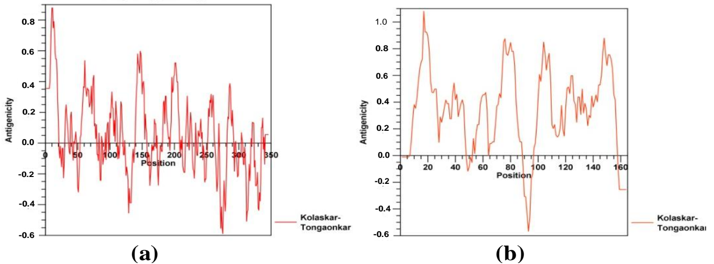
Figure 1. Antigenicity plots of common proteins causing diarrheal diseases. (a) ompA; (b) lspA; (c) Lpp; (d) Pal; (e) VacJ; (f) YaeC; (g) feoB.
