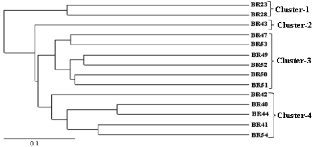
Figure 1. Cluster analysis of the 14 rice genotypes using distant coefficient.
