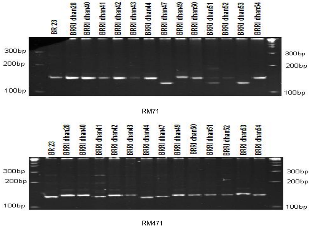
Figure 2. Banding pattern of the 14 rice genotypes generated by primer RM71 and RM471.
