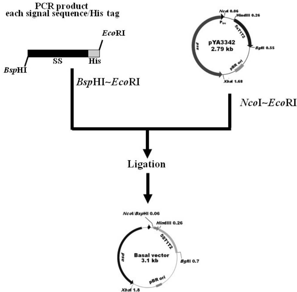
Figure 1. Schematic diagram of strategy for cloning of signal sequence (SS) DNA. The signal sequences of Bla ( \beta -lactamase), AgfA (thin aggregative fimbriae A), StfA S. typhimurium fimbriae A) and OmpW (outer membrane protein W) were used in this study. Each PCR-amplified Bsp HI- Eco RI SS DNA was cloned into pYA3342 digested with Nco I and Eco RI. Gray box indicates a His 6 -tag contained at the C-terminus of each SS.
