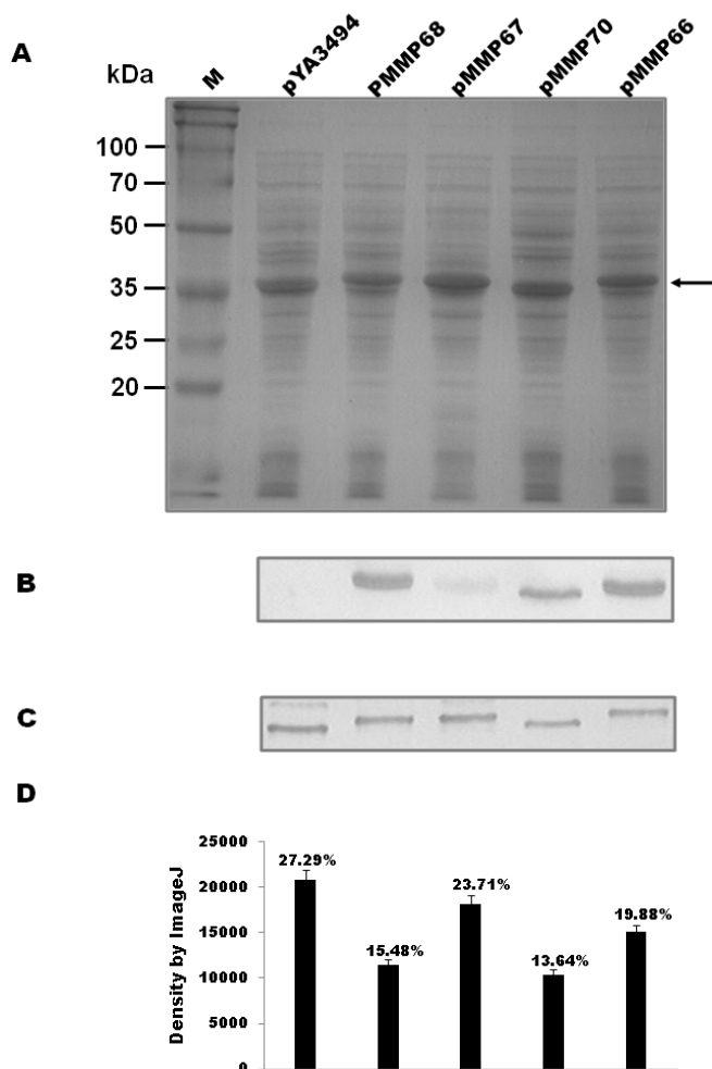
Figure 3. Expression of PspA in S. typhimurium containing recombinant plasmids. S. typhimurium strains harboring pYA3494, pMMP66, 67, 68 and 70 were grown in LB broth until exponential phase (0.8 at OD 600 ). Equal amounts of cell lysates were subjected to SDS-PAGE followed by immunoblot analyses with specific antibodies for each component. The goat anti-mouse conjugated with HRP was used as the 2nd antibodies. (A) SDS-PAGE of total lysates. Separated bands were visualized by Coomassie staining. (B to C) immunoblot of total lysates. His 6 -tagged SS was detected by monoclonal antibody specific for His 6 -tag (B), and expressed PspA protein was detected by monoclonal antibody specific for PspA (C). (D) Quantitative analysis of PspA protein. Relative immuno-reactive intensities were analyzed by imageJ program. Arrow indicates the PspA protein.
