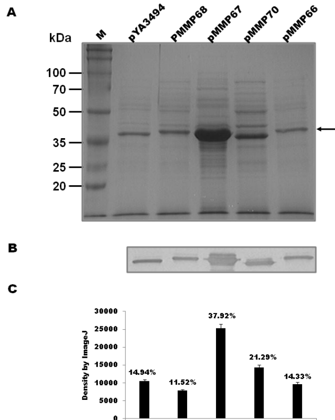
Figure 4. Immunoblot of secreted PspA proteins. S. typhimurium \chi 8554 harboring plasmids were cultured in LB broth until exponential phase (0.8 at OD 600 ). Equal amount of cell-free culture supernatant were subjected to SDS-PAGE and immunoblot analyses. (A) SDS-PAGE analysis. Separated bands were visualized by Coomassie staining. (B) Immunoblot of secreted proteins. The PspA protein was detected by monoclonal antibody specific for PspA. (C) Quantitative analysis of PspA protein. Relative immuno-reactive intensities were analyzed by imageJ program. Arrow indicates the PspA protein.
