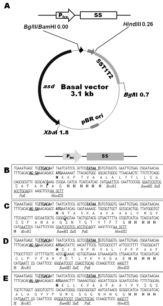
Figure 2. Genetic maps of recombinant plasmids. The physical maps of each recombinant plasmid are indicated with their representative restriction enzyme sites: (A) Basal vector, (B) pMMP62, (C) pMMP63, (D) pMMP64 and (E) pMMP65. The P_{trc} promoter region, ribosome binding site (RBS), each SS, His 6 -epitope and multi-cloning sites (MCS) are revealed in enlarged box. Unique enzyme sites in MCS are designated by underlined bold letters. P_{trc} , trc promoter; 5SST1T2, 5S rRNA terminator; “ asd ”, aspartate semialdehyde dehydrogenase gene; SS, OmpW SS (B), StfA SS (C), Bla SS (D) and AgfA SS (E).
