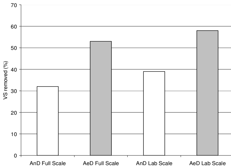
Figure 1. Percent of volatile solids removed during aerobically digested (AeD) and anaerobically digested (AnD) sludge for both full and lab scale experiments.
