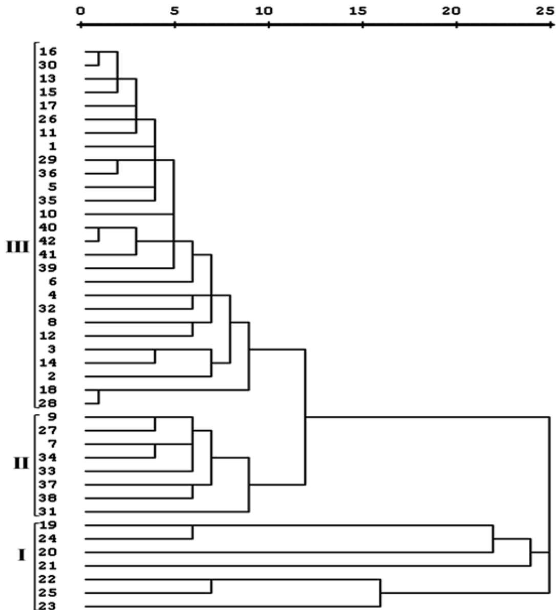
Figure 1. Dendrogram of 42 populations of faba bean from southern Tunisia based on sixteen characteristics using Neighbor-joining method.
