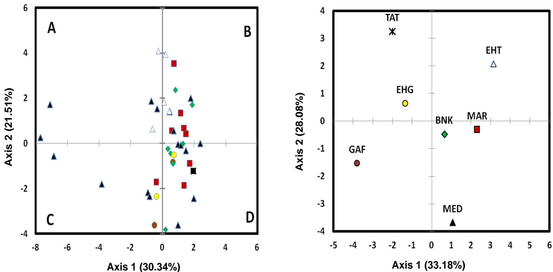
Figure 2. The Principal components analysis of forty two populations based on the sixteen characteristics. Codes indicate populations and oasis of origin: (■) Mareth, (●) El Hamma (Gabes) , (●) Gafsa, (△) El Hamma (Tozeur), (▲) Medenine, (◆) Beni Khedache and (×) Tataouine.
