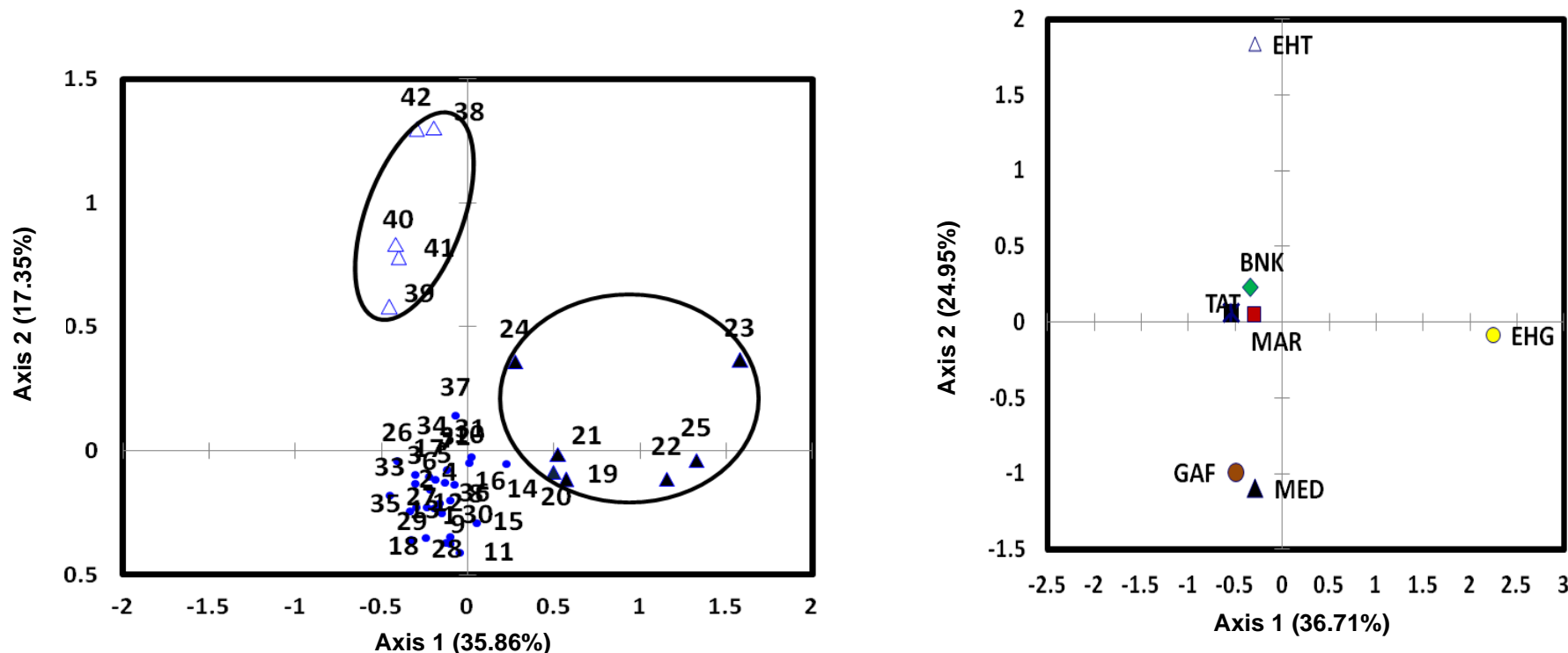
Figure 3. The Multiple Components Analysis of forty two populations based on the nineteen qualitative characteristics.
