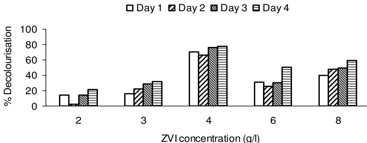
Figure 4. Effect of zero valent iron (ZVI) concentration on decolourisation of Reactive Blue 2 (100 mg/l) with SRB's in untreated sludge.
