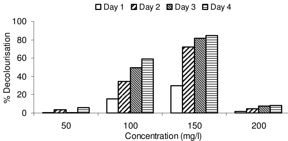
Figure 3. Effects of different concentration of Reactive Blue 2 on decolourisation by sulphate reducing bacteria in untreated sludge.
