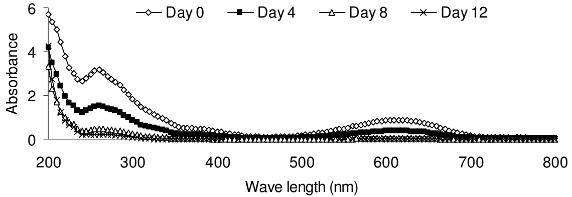
Figure 1. Typical changes in absorbance peaks monitored in a bioreactor for the anaerobic degradation and decolourisation of Reactive Blue 2 (100 mg/l) by sulphate reducing bacteria in untreated sewage sludge.
