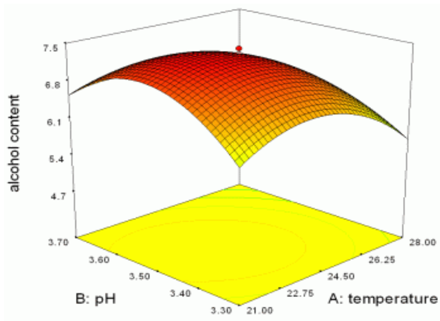
Figure 1. Response surface plots of ethanol (%) showing the interactive effect of temperature and pH.
