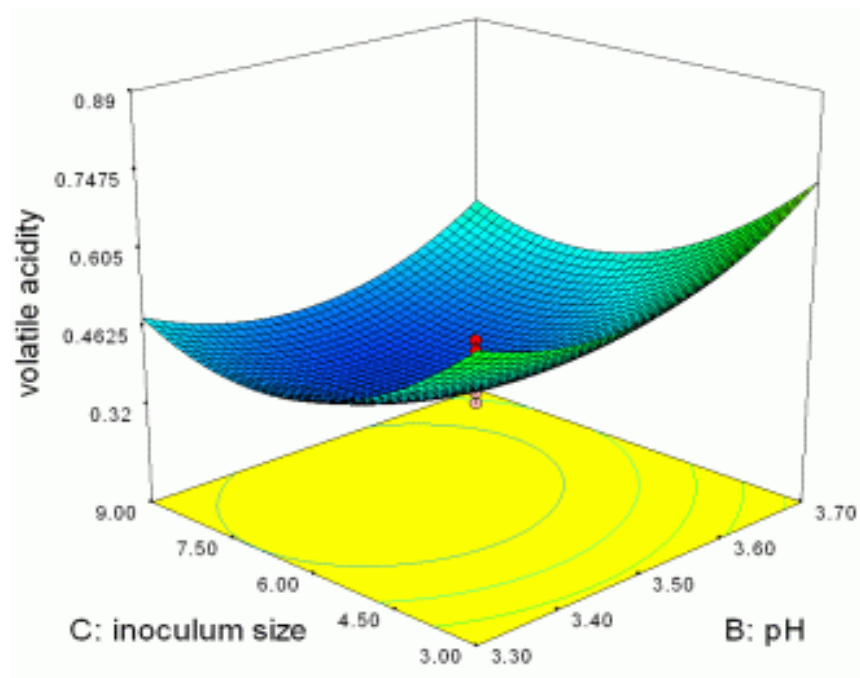
Figure 6. Response surface plots of volatile acidity ( \text{g l}^{-1} ) showing the interactive effect of pH and inoculum size.
