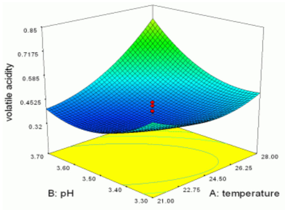
Figure 4. Response surface plots of volatile acidity ( \text{g l}^{-1} ) showing the interactive effect of temperature and pH.
