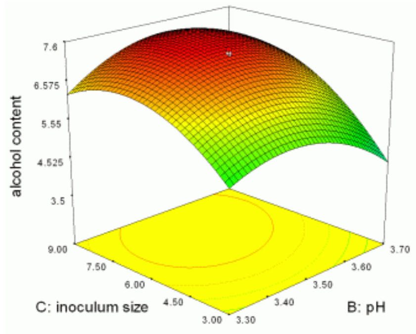
Figure 3. Response surface plots of ethanol (%) showing the interactive effect of pH and inoculum size.
