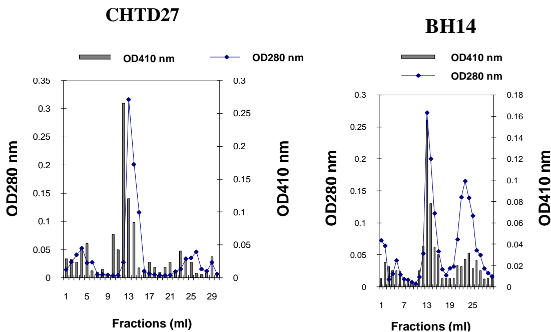
Figure 4. DEAE Cellulose Chromatograms of G100 fractions. Absorbance of protein contents was measured at 280 nm and of AP activity at 410 nm.
