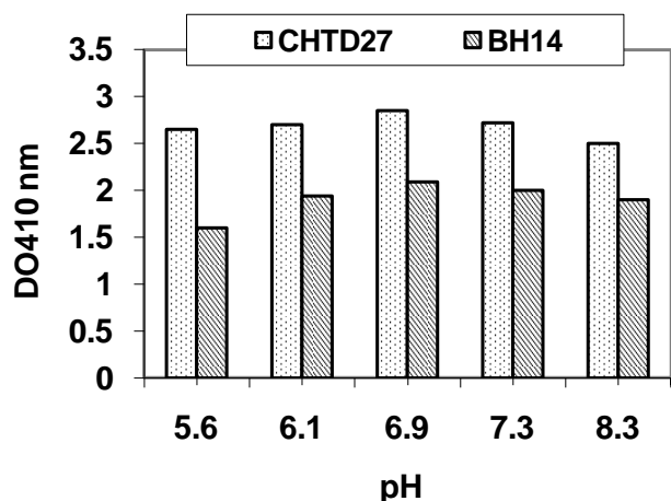
Figure 1. Effect of pH on cells AP activities.
