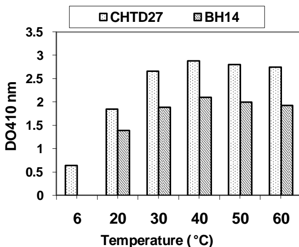
Figure 2. Effect of temperature on cells AP activities.
