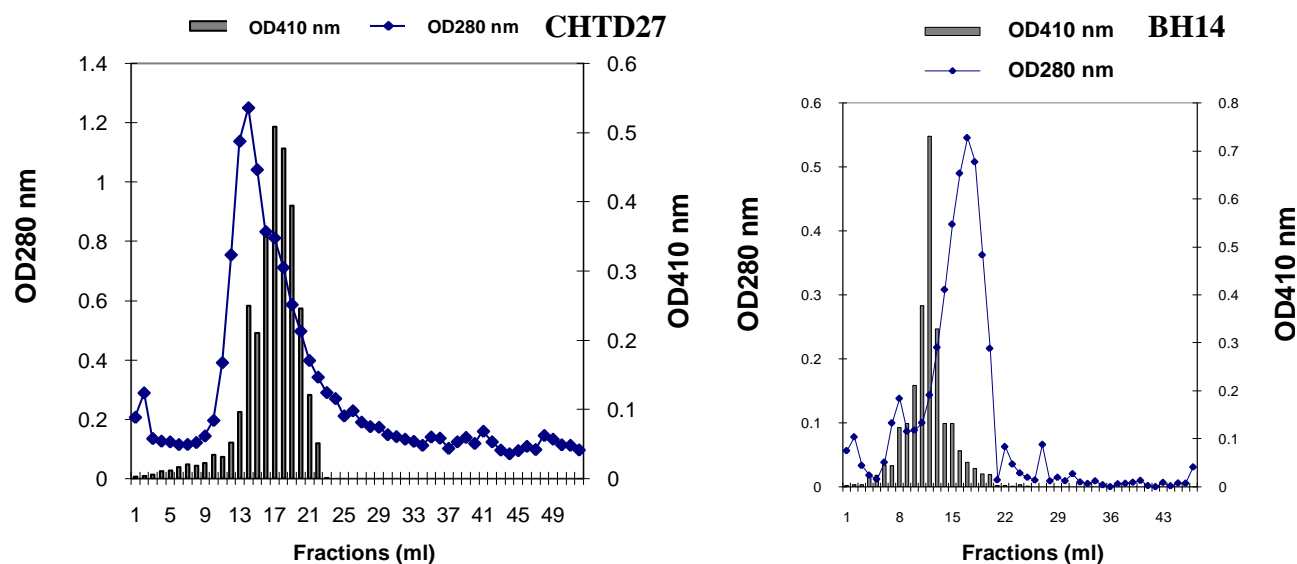
Figure 3. Séphadex G100 chromatograms of SA 80 fraction. Absorbance of protein contents was measured at 280 nm and of AP activity at 410 nm.
