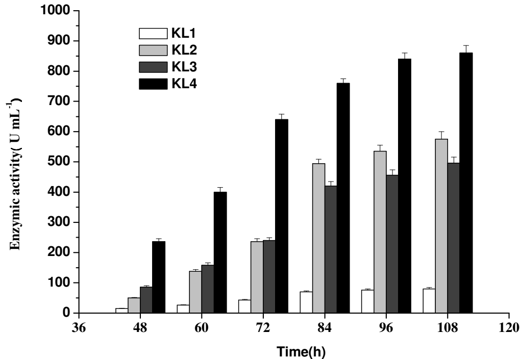
Figure 1. Comparison of enzymic activity of recombinant chymosin produced by KL1, KL2, KL3 and KL4 at various culture stages.
