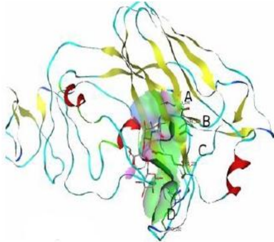
Figure 1. Docking visualization of HA with sialic acid. A, Ile_225; B, Val_226; C, Lys_228; D, Arg_232. Figure taken from Usman et al. (2010), Figure 4.
