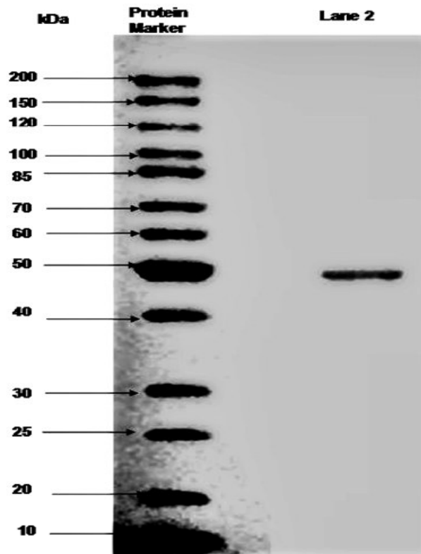
Figure 2. Reducing SDS-PAGE analysis of the purified amidase shown in Lane 2.
