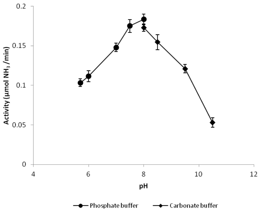
Figure 3. Effect of pH on the activity of purified amidase.
