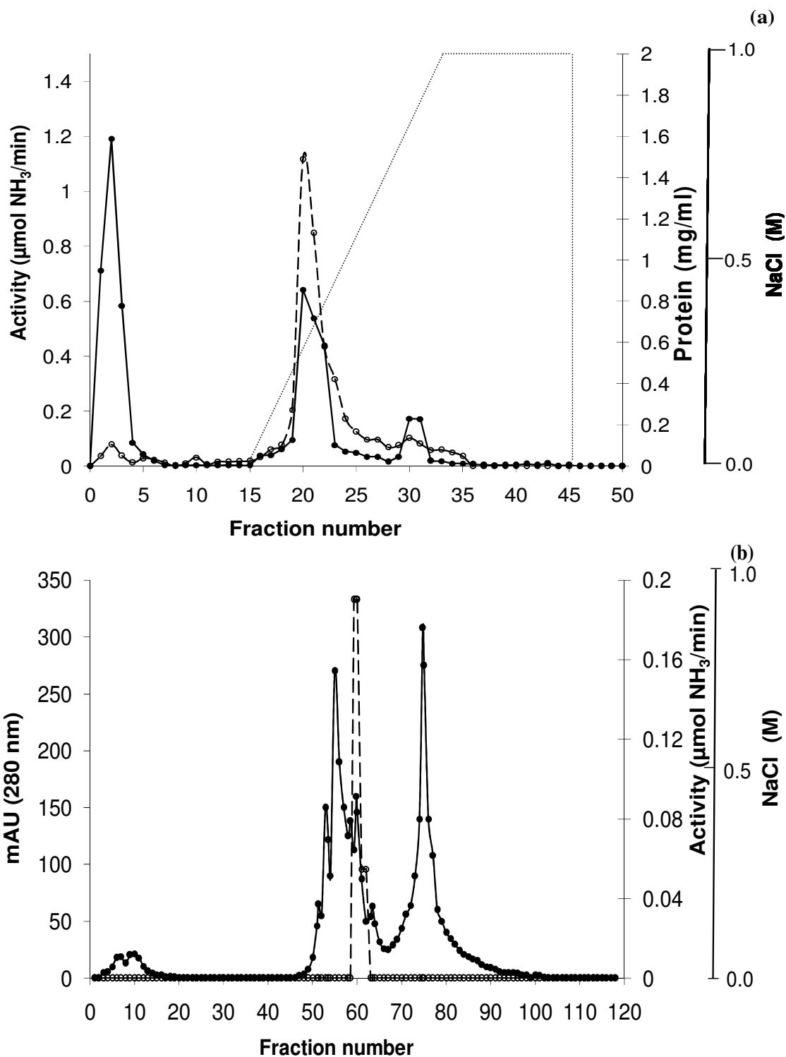
Figure 1. Amidase elution profile using (a) DEAE-cellulose anion exchanger column, (b) Mono-Q™ strong-anion exchanger column and (c) Zorbax® Bioseries GF-250 gel filtration column. -o-, Amidase activity; -•-, protein; ..... gradient of 1M NaCl were measured during purification steps.
