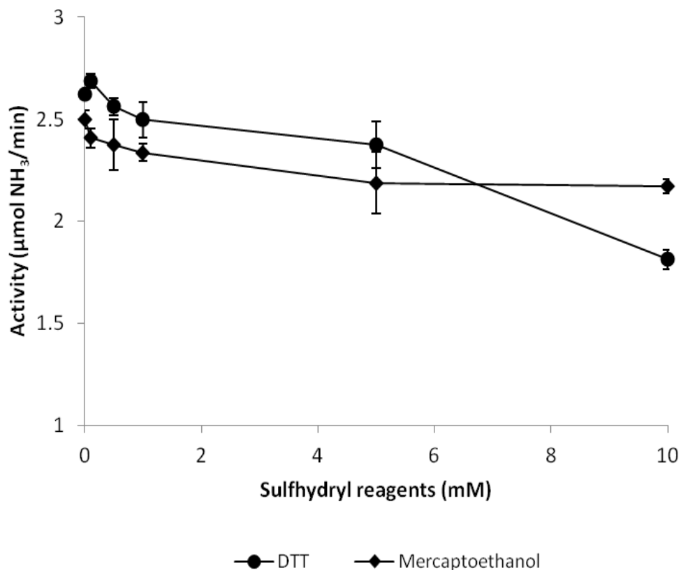
Figure 5. Effect of sulfhydryl reagents on amidase activity.
