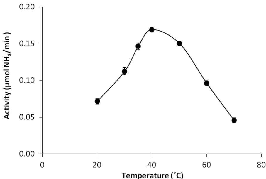
Figure 4. Effect of temperature on the activity of purified amidase.
