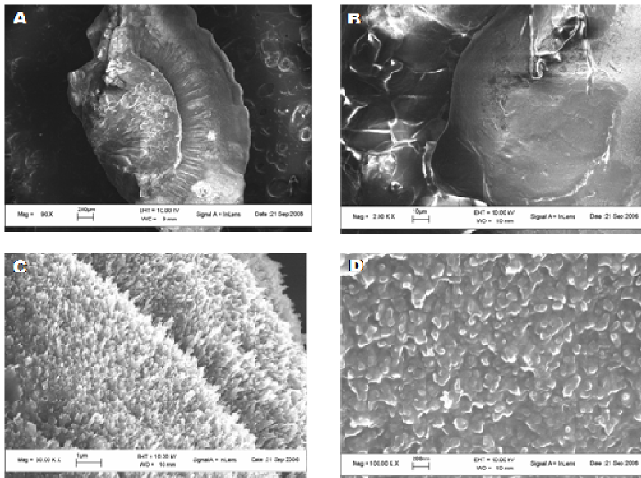
Figure 3. The crystal structure of carp otoliths through scanning electric microscope analysis. (a) The reverse side of asteriscus otoliths showing the microstructure of annual growth increments. (b) The original growth of asteriscus, showing irregular and variable microstructure. (c) The surface structure of asteriscus after EDTA etching. (d) The original surface structure of asteriscus without EDTA etching. EDTA, Ethylene diamine tetra-acetic acid.
