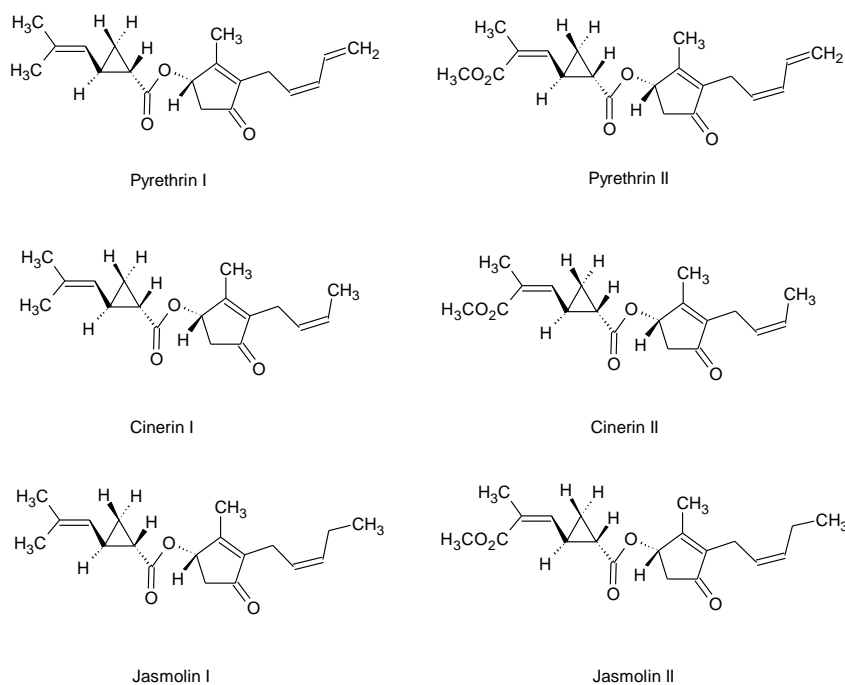
Figure 1. Chemical structure of individual pyrethrins.
