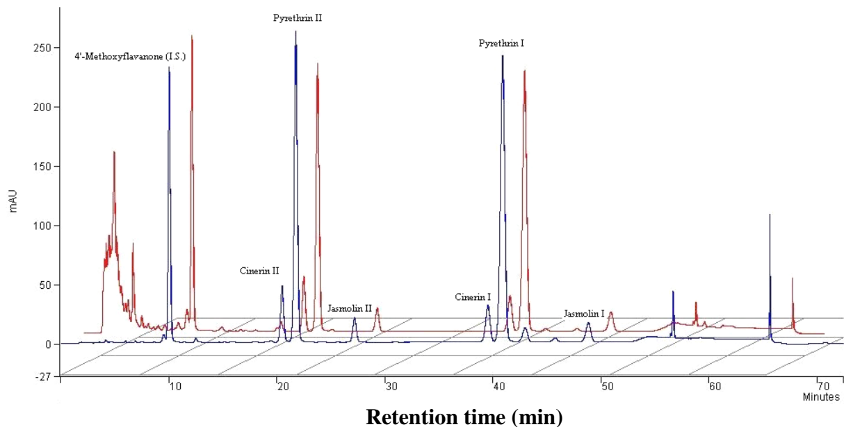
Figure 2. Reversed-phase HPLC chromatogram of standard (blue line) and sample (red line) of pyrethrum extract. (Mobile phase flow rate 1 \text{ mL min}^{-1} , injection volume 20 \mu\text{L} , UV detector at 230 \text{ nm} )
