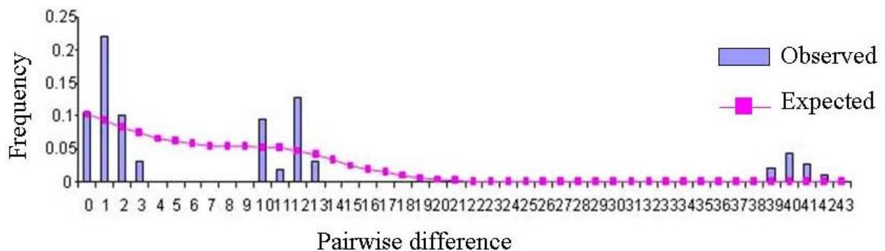
Figure 4. Mismatch distribution analysis for LAG population of C. nigrodigitatus .
