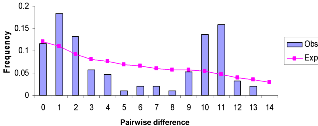
Figure 3. Mismatch distribution analysis for Epe population of C. nigrodigitatus .
