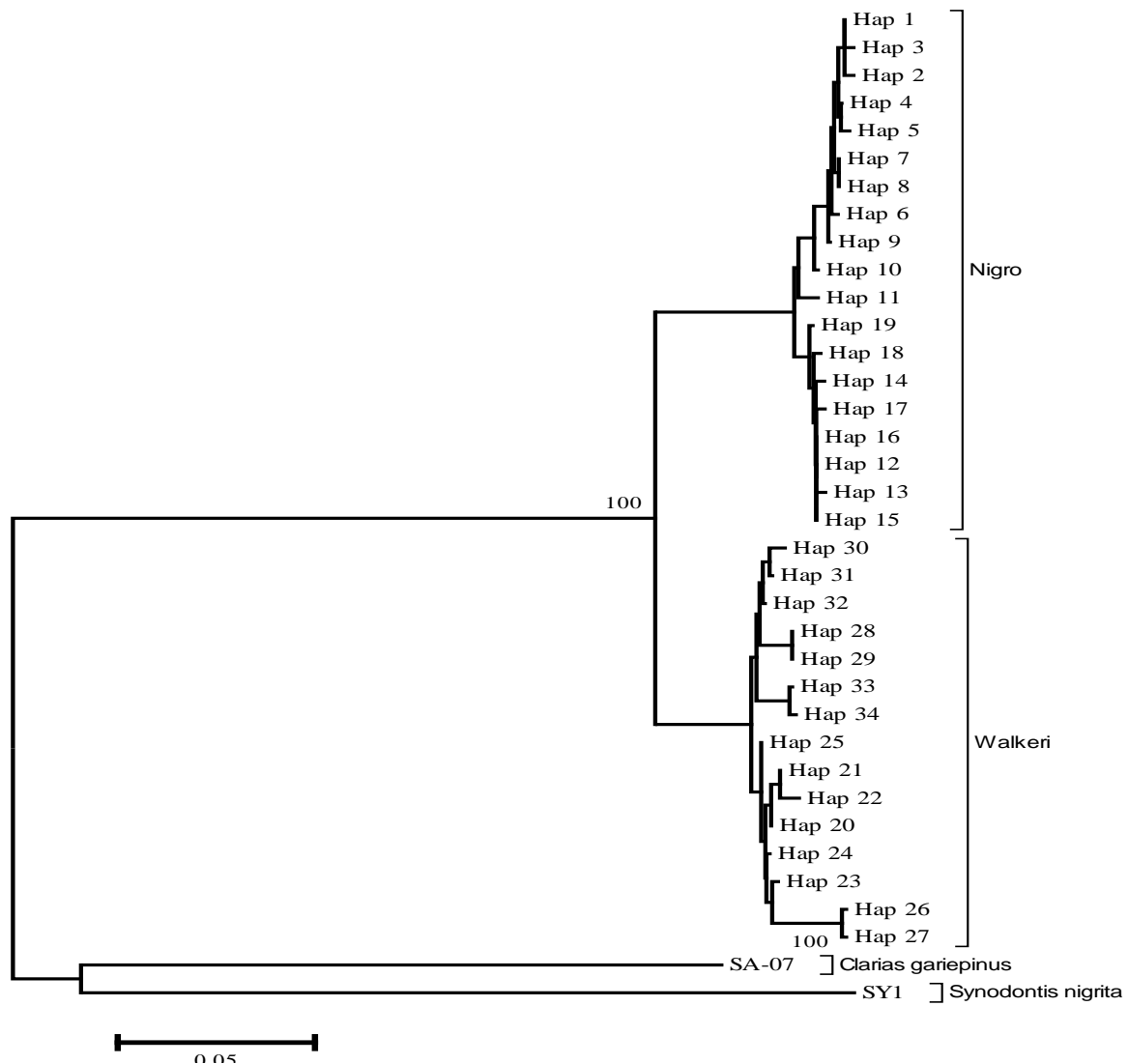
Figure 2. Neighbour-joining tree constructed using Tamura-Nei distances for 34 control region haplotypes of C. nigrodigitatus (Nigro) and C. walkeri (WAK) from the Lagos Lagoon complex.
