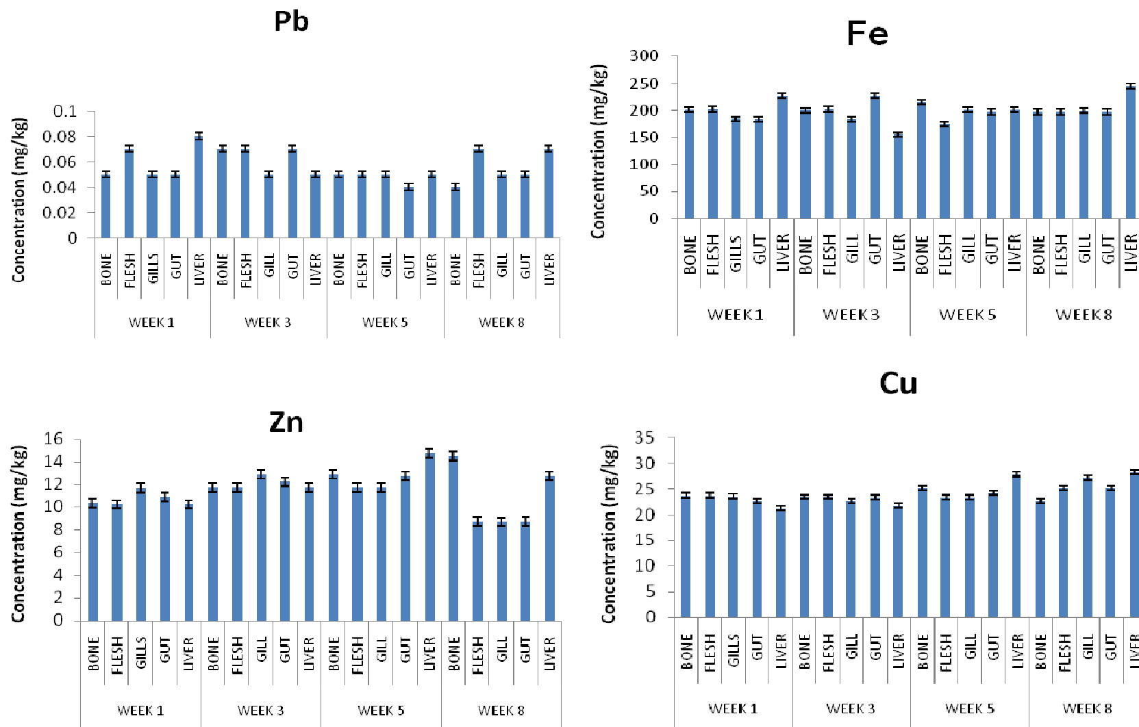
Figure 2. Concentrations of heavy metals in fish organs with time.
