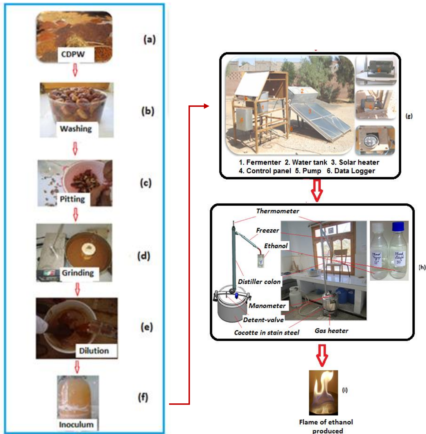
Figure 2. Bioethanol generation process.
