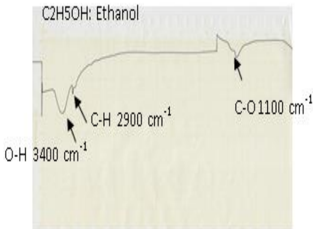
Figure 5. Vibration sign of the ethanol produced.
