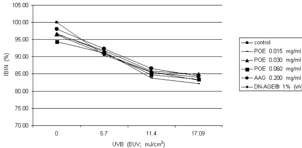
Figure 1. Percentage of IBIN on pre-treated KSCs after receiving irradiation at different UVB-doses (EUV; 0-17.09 mJ/cm 2 ).
