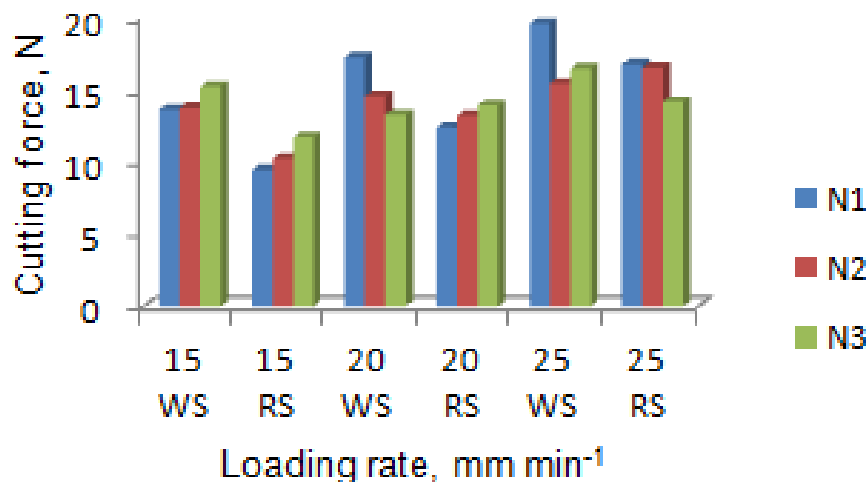
Figure 11. Influence of cutting force of WS and RS at different internode position under loading rates.
