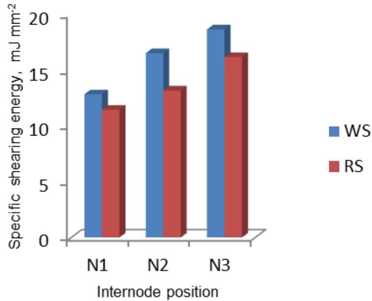
Figure 8. Influence of specific shearing energy of WS and RS at different internode position under 20 mm min -1 .
