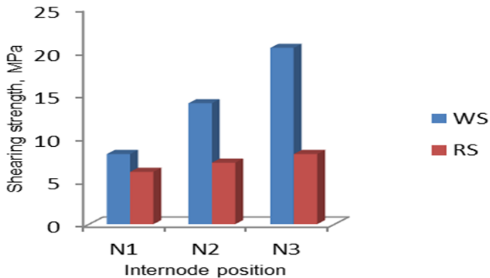
Figure 4. Shear strength of WS and RS at different internode positions under 15 \text{ mm min}^{-1} .
