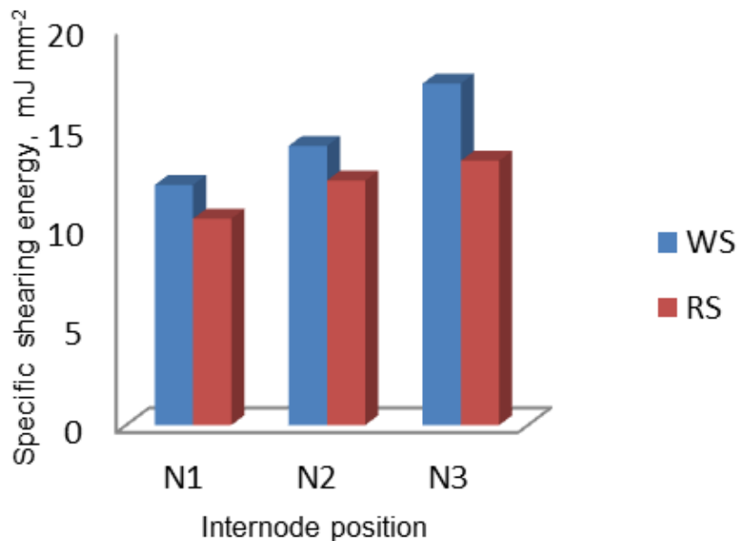
Figure 7. Influence of specific shearing energy of WS and RS at different internode position under 15 \text{ mm min}^{-1} .
