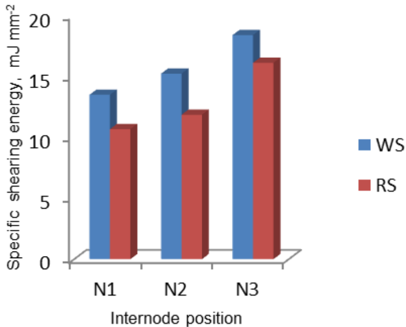
Figure 9. Influence of specific shearing energy of WS and RS at different internode position under 25 mm min -1 .
