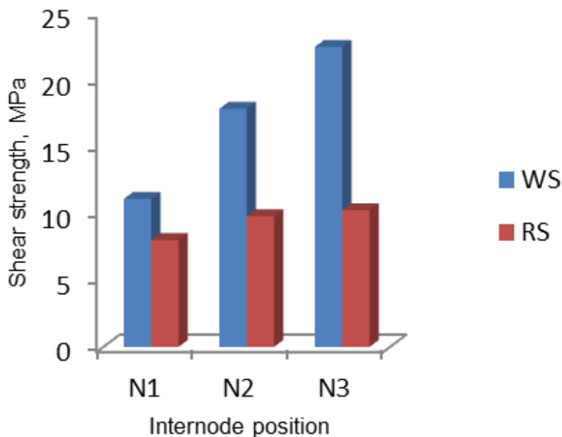
Figure 5. Shear strength of WS and RS at different internode positions under 20 \text{ mm min}^{-1} .
