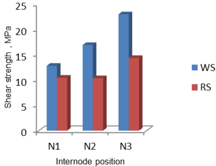
Figure 6. Shear strength of WS and RS at different internode positions under 25 \text{ mm min}^{-1} .
