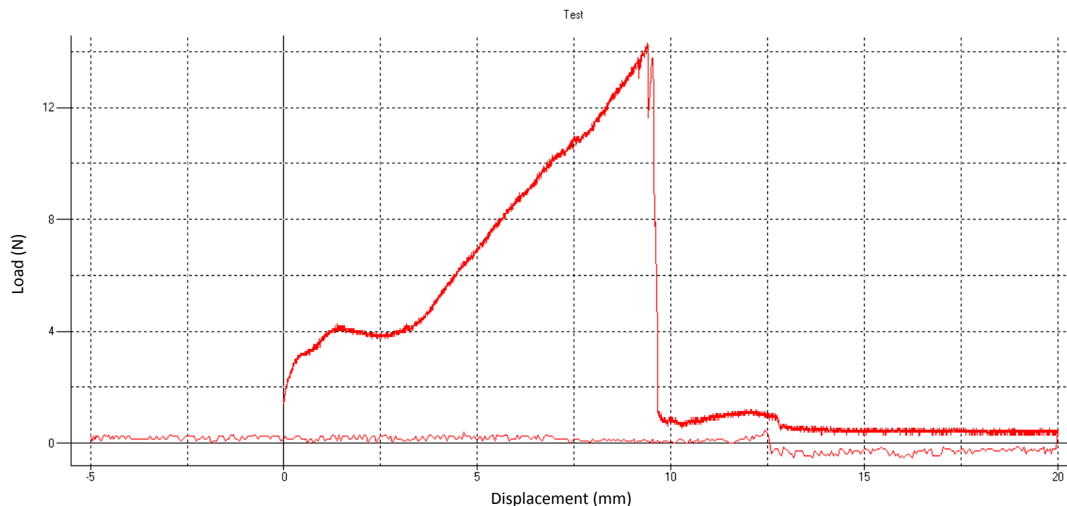
Figure 10. The cutting force versus displacement curve for WS.
