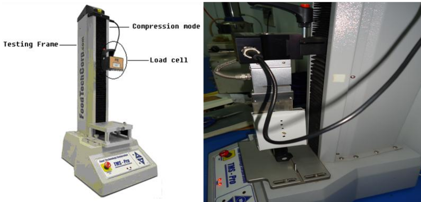
Figure 1. A TMS-Pro texture analyzer testing machine used to measure the shear strength and cutting force of WS and RS.
