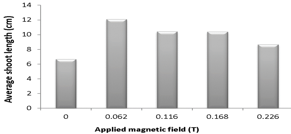
Figure 3. Variation of average shoot length (8 day old) with applied magnetic field.
