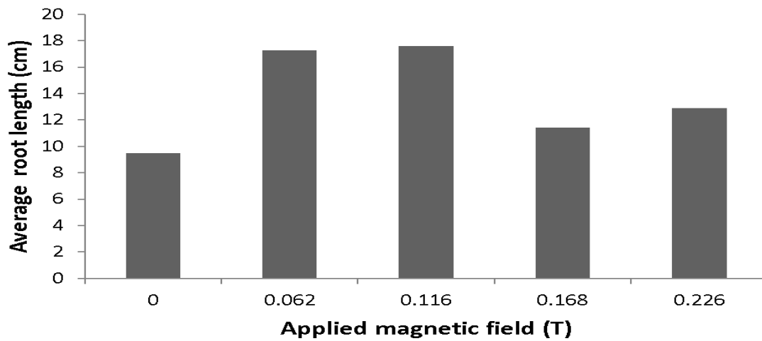
Figure 4. Effect of applied magnetic field on average root length (8 day old).
