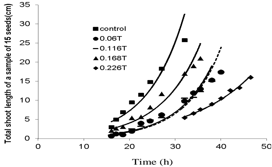
Figure 6. Exponential variation of total shoot length of a sample of 15 seeds with time.
