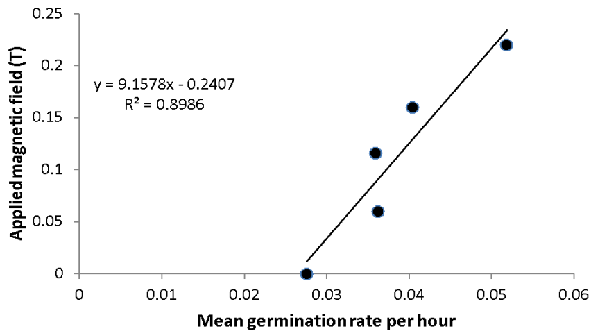
Figure 7. Variation of germination rate GR_g or 1/t_g as a linear function of applied magnetic field B.
