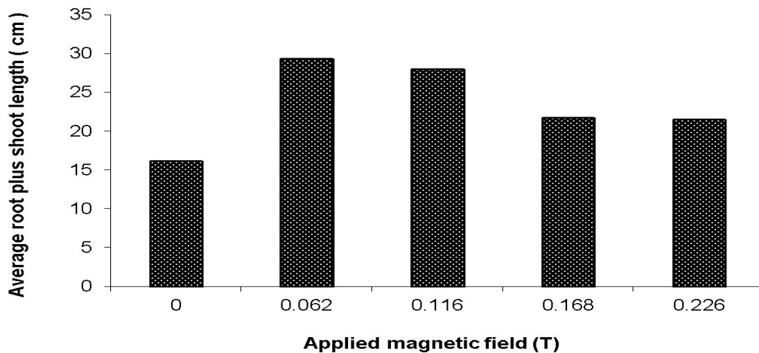
Figure 5. Effect of applied magnetic field on average root length plus shoot length (8 day old).
