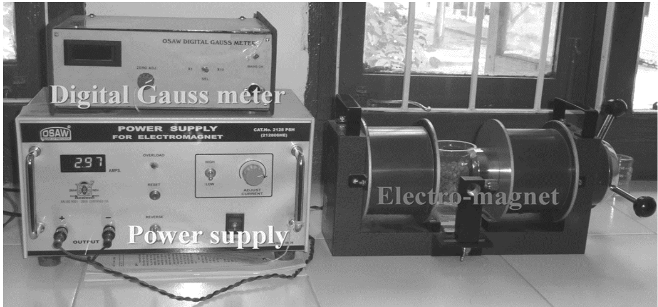
Figure 1. Photograph of magnetic field generator.
