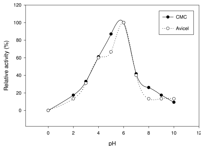
Figure 3. Optimum pH of GST-CBHI.1 on CMC and Avicel.
