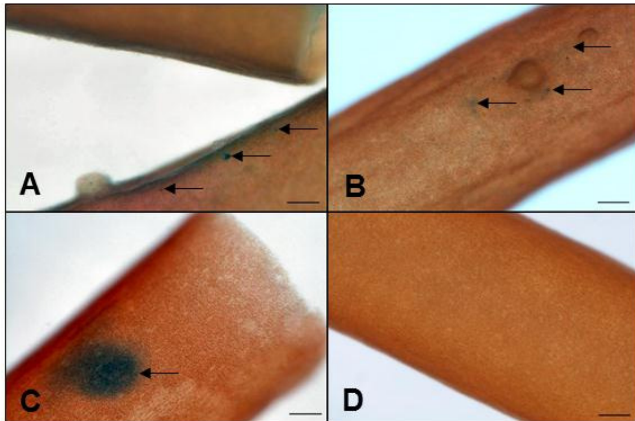
Figure 1. Histological lacZ assay. G. gracilis thalli (2 days post-bombardment) with blue-stained areas (arrows) indicating \beta -galactosidase activity in the samples bombarded with pCaMV- \beta -Gal (A); pCMV- \beta -Gal (B); pSV- \beta -Gal (C) bombarded thallus; and, gold particles lacking vector DNA (negative control) (D). Scale bar = 100 \mu m (A-D).
