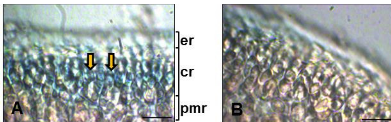
Figure 2. Sectioned G. gracilis thalli stained two days post-bombardment. pSV- \beta -Gal-bombarded thallus exhibited blue staining (arrows) within cells located in the cortical region (cr), which lies between the epidermal (er) and perimedullary (pmr) regions (A), while thalli bombarded with gold particles lacking vector DNA (negative control) showed no blue staining (B). The sections were viewed and photographed under a Nikon Eclipse 50i compound microscope. Scale bar = 40 \mu m.
