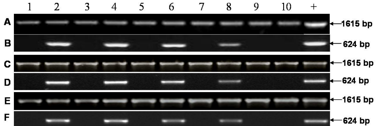
Figure 3. PCR analysis of total DNA isolated from bombarded thalli. Lanes 1, 3, 5, 7 and 9 show seaweed bombarded with non-DNA-attached gold particles (negative control) sampled 1, 2, 3, 5 and 7 post-bombardment, respectively; lanes 2, 4, 6, 8 and 10 show plasmid-bombarded seaweed (test sample) sampled 1, 2, 3, 5 and 7 days post-bombardment, respectively; + indicates a positive control. Panels A, C and E: DNA fragments amplified with G. gracilis 18S rRNA gene specific primers in samples bombarded with pSV- \beta -Gal, pCaMV- \beta -Gal and pCMV- \beta -Gal, respectively. Panels B, D and F: DNA fragments amplified with lacZ specific primers in samples bombarded with pSV- \beta -Gal, pCaMV- \beta -Gal and pCMV- \beta -Gal, respectively.
