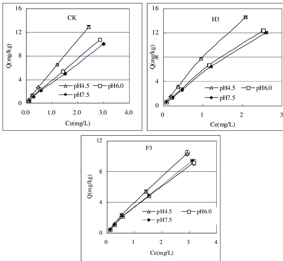
Figure 4. Adsorption of imidacloprid under different pH conditions (n = 3).
