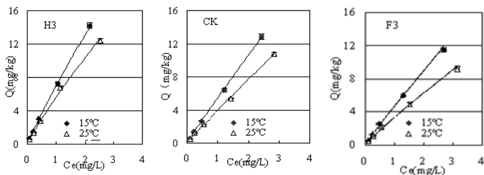
Figure 3. Sorption isotherms for imidacloprid on soils ( n = 3 ). H3 and F3 refer to exogenous HA and FA added to soil to enhance the amount of soil organic carbon (SOC) by 10.0 \text{ g kg}^{-1} , respectively.
