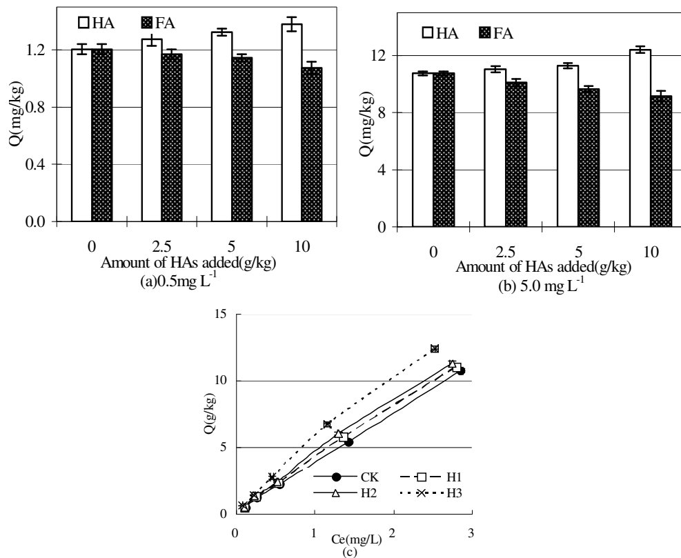
Figure 2. Adsorption of imidacloprid in differently treated soils ( n = 3 ). H1, H2, and H3 were exogenous HA added to soil to enhance the amount of soil organic carbon (SOC) by 2.5, 5.0 and 10.0 \text{ g kg}^{-1} , respectively.
