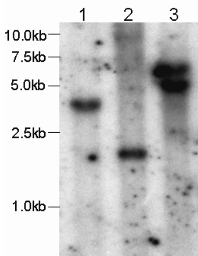
Figure 3. Southern blot analysis of HbCCH1 . Rubber tree genomic DNA was digested with EcoRI (1), BamHI (2) and Hind III (3), followed by hybridization with ^{32}\text{P} -labeled HbCCH1 ORF.
