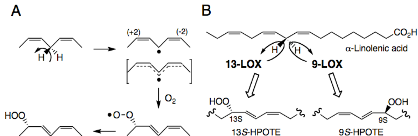
Figure 2. LOX reaction showing the principal steps of LOX reaction (Panel A), and the actual reactions of plant LOXs and \alpha -linolenic acid (Panel B). HPOTE: Hydroperoxyoctadecatrienoic acid (Chedea and Jisaka, 2011).
