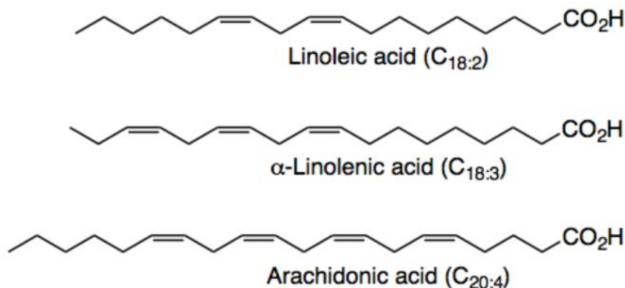
Figure 1. Lipoxygenase substrates, linoleic, α- linolenic and arachidonic acid.
