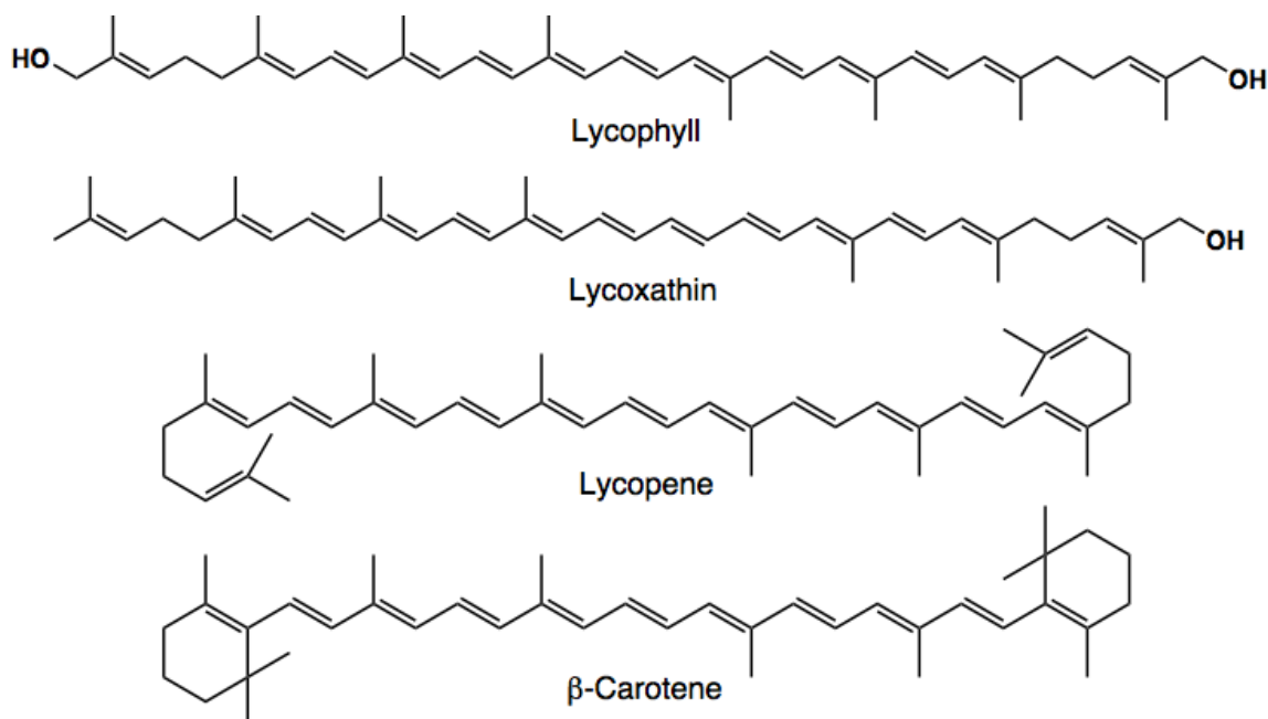
Figure 3. Carotenoids oxidized by lipoxygenase.
