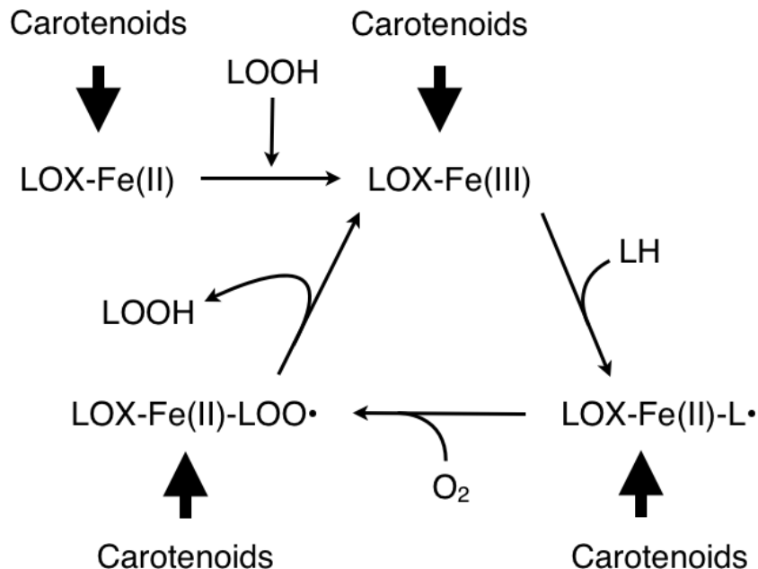
Figure 4. Possible interactions of carotenoids with lipoxygenase pathway.
