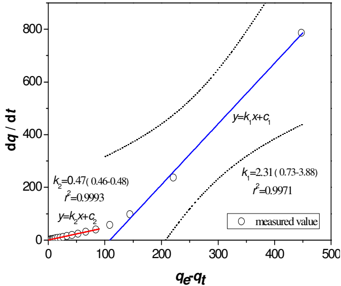
Figure 5. Adsorption rate constants in two-step adsorption kinetics model on H103 resin.
