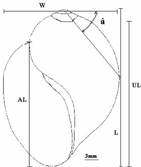
Figure 2. Drawing to show dimensions of the shell illustrated for a specimen of Bulinus sp. Shell length (L); aperture length (AL); ultimate whorl length (UL); shell width (W) and apical angle ( \hat{a} ). Scale bar= 3mm.
