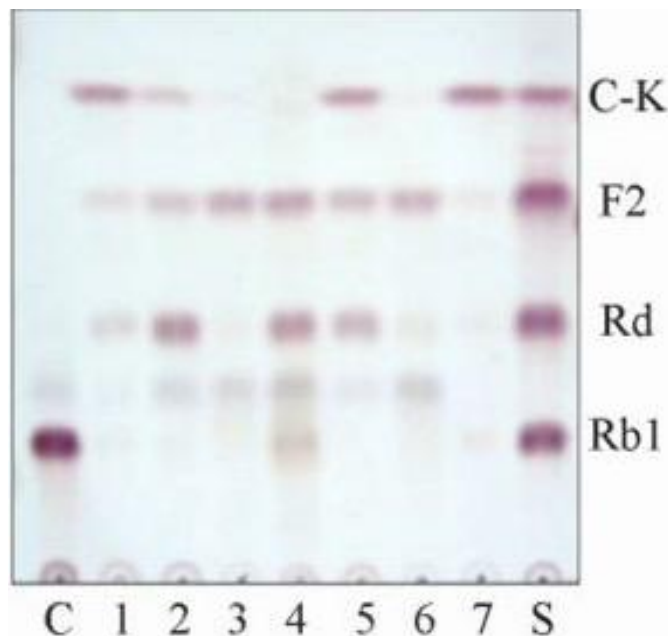
Figure 1. TLC analysis of conversion products of ginsenoside Rb1 by GH9 in different media. Lane 1, H 2 O; lane 2, NB; lane 3, YM; lane 4, MRS; lane 5, R2A; lane 6, LB; lane 7, YB; lane C, control; lane S, saponin standards.
