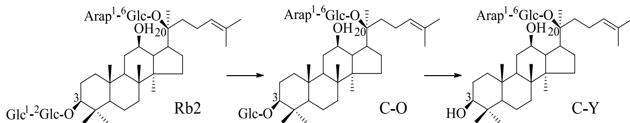
Figure 8. The mechanism by which GH9 converts Rb2 into C-Y.
