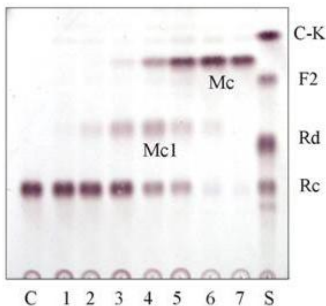
Figure 9. TLC analysis of GH9 conversion of ginsenoside Rc. Lane C, control; lane S: standard.
