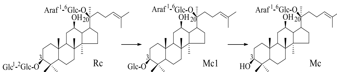
Figure 10. The mechanism by which GH9 converts Rc into Mc.
