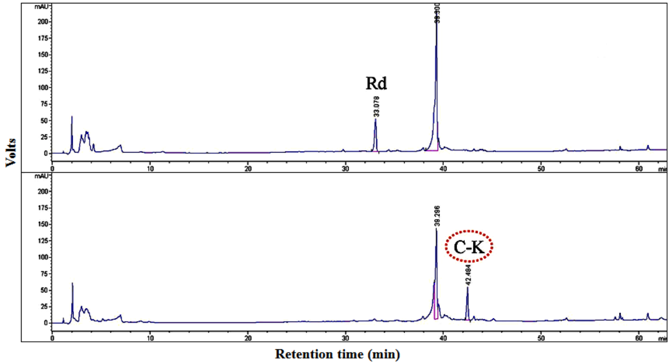
Figure 13. HPLC analysis of GH9 conversion of ginsenoside Rd.
