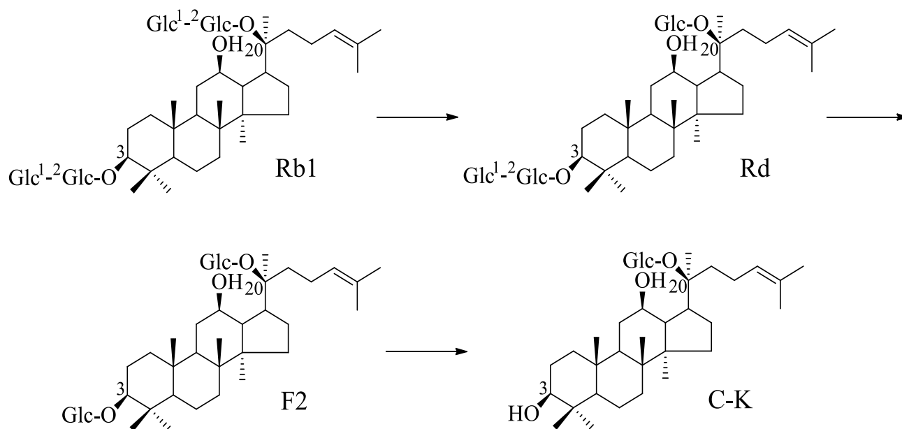
Figure 5. The mechanism by which GH9 converts Rb1 into C-K.
