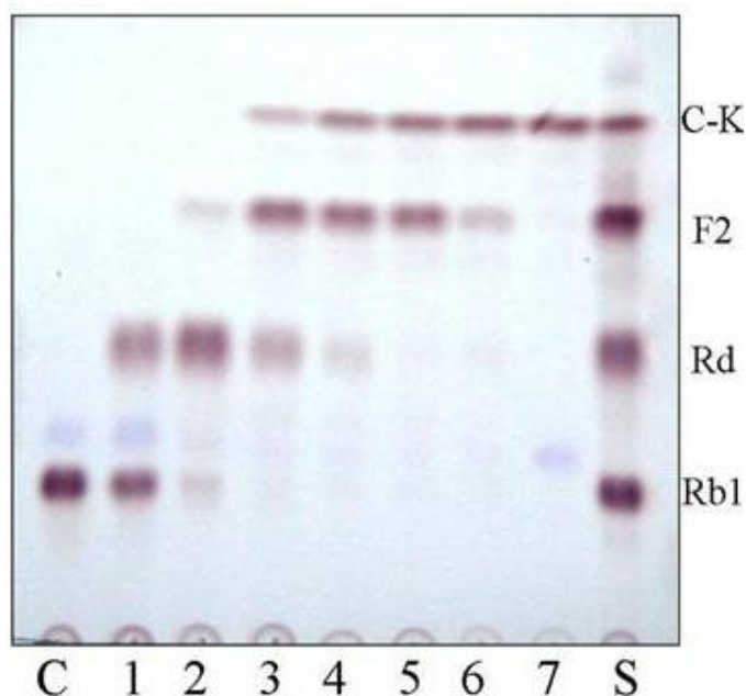
Figure 4. TLC analysis of GH9 conversion of ginsenoside Rb1. Lane C, Control; lane S, saponin standards.
