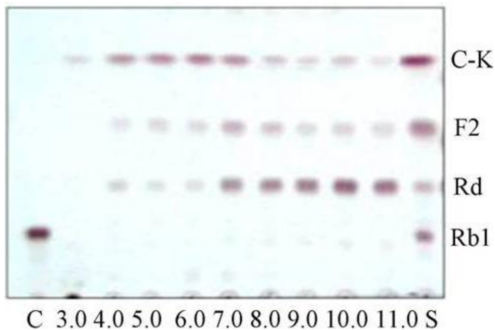
Figure 2. TLC results of the conversion products of ginsenoside Rb1 by GH9 at pH values from 3.0 to 11.0. Lane C, Control; lane S, saponin standard.
