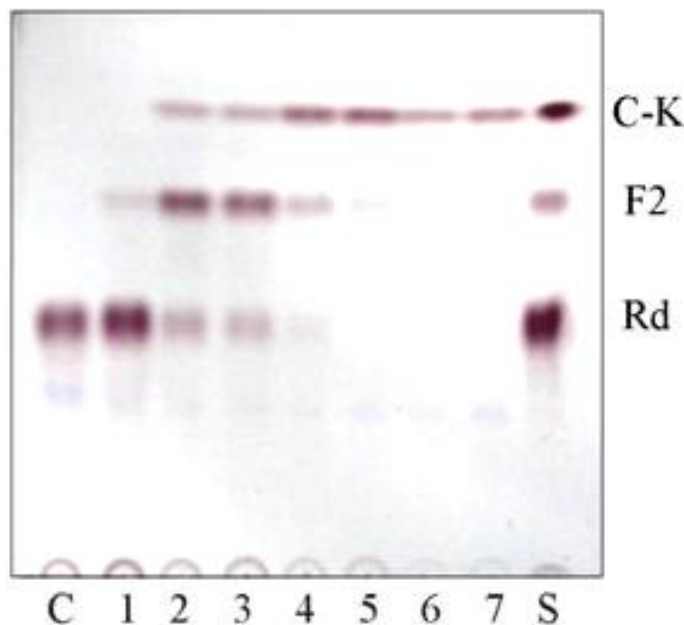
Figure 11. TLC analysis of GH9 conversion of ginsenoside Rd. Lane C: control; lane S: saponin standards.
