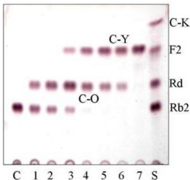
Figure 7. TLC analysis of GH9 conversion of ginsenoside Rb2. Lane C, Control; lane S, saponin standard.
