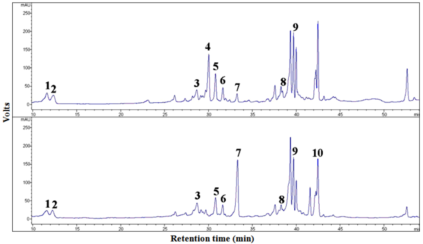
Figure 14. HPLC analysis results of GH9 conversion of total ginsenoside leaching agent. 1, Rg1; 2, Re; 3, Rh1; 4, Rb1; 5, Rc; 6, Rb2; 7, Rd; 8, F2; 9, Rg3; 10, C-K.
