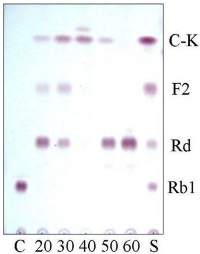
Figure 3. TLC analysis of the conversion products of ginsenoside Rb1 by GH9 under different temperatures. Lane C, Control; lane S, saponin standard.
