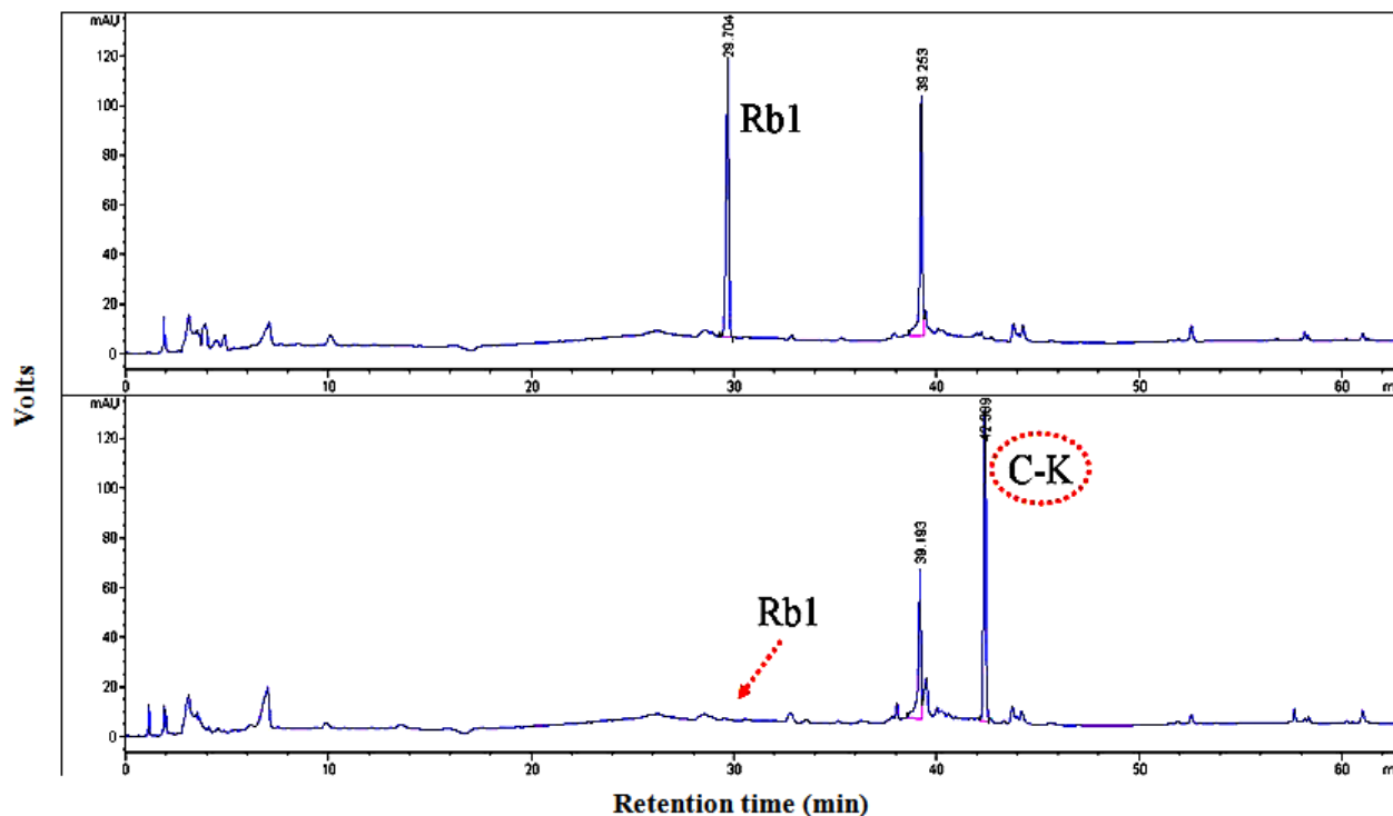
Figure 6. HPLC analysis of GH9 conversion of ginsenoside Rb1.
