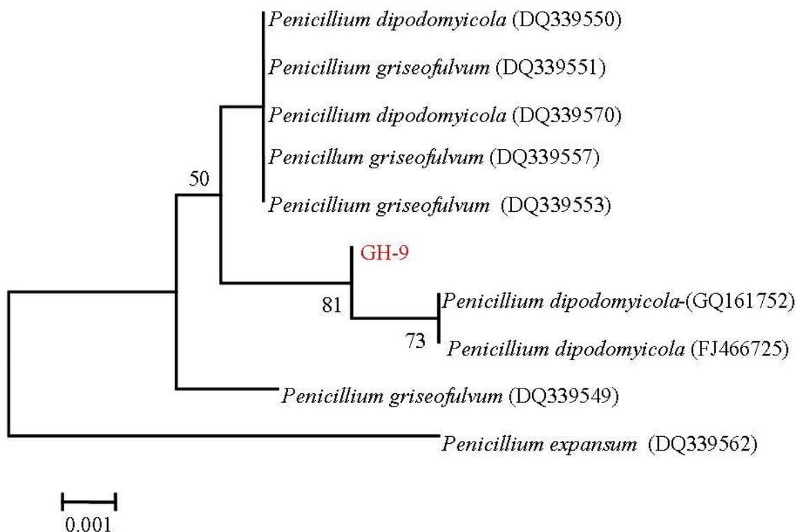
Figure 16. A phylogenetic tree based on the ITS rRNA gene sequences, showing the phylogenetic relationships of the strain GH9.
