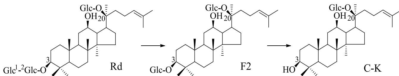
Figure 12. The mechanism by which GH9 converts Rd into C-K.
