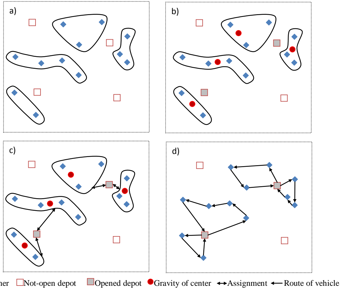
Figure 1. Illustrative example for the proposed heuristic method.
