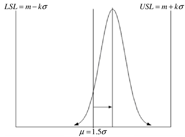
Figure 1. The process mean shifts 1.5\sigma right chart.
