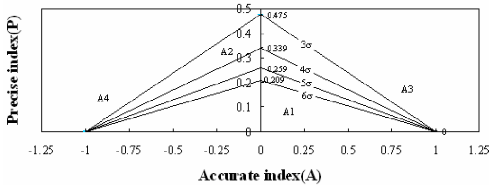
Figure 2. The PCAC chart which the quality level is from 3 to 6σ.
