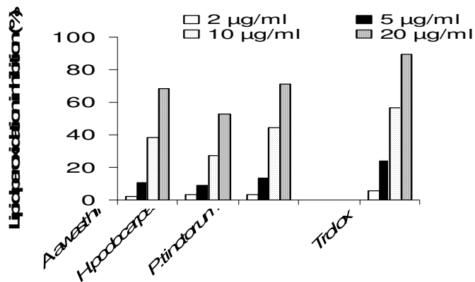
Figure 1. Lipid peroxidation inhibition by the extract of various concentrations of the one year old cultured symbionts of lichen species. Data plotted are mean of five consecutive readings.
