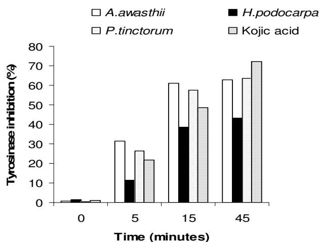
Figure 5. The rate of tyrosinase inhibition under various time period by the extract (20 \mu\text{g/ml} ) of one year old cultured symbionts of lichen species. Kojic acid a commercial tyrosinase inhibitor used for comparison. Data plotted are mean of five consecutive readings.
