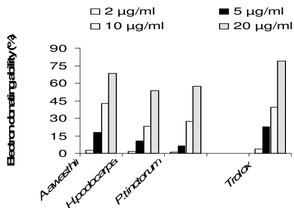
Figure 3. Electron donating ability by the extract of various concentrations of one year old cultured symbionts of lichen species. Trolox a water soluble vitamin E analogue used as commercial antioxidant for comparison. Data plotted are mean of five consecutive readings.
