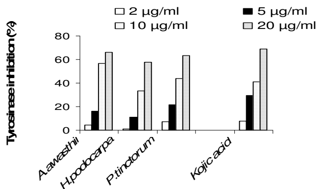
Figure 4. Tyrosinase inhibition by the extract of various concentrations of one year old cultured symbionts of lichen species. Kojic acid used as standard tyrosinase inhibitor for the comparison. Data plotted are mean of five consecutive readings.
