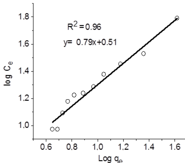
Figure 9. Linearized Freundlich isotherm (initial dye concentration = 103 mg/ L, pH = 7-9, temperature = 24°C).
