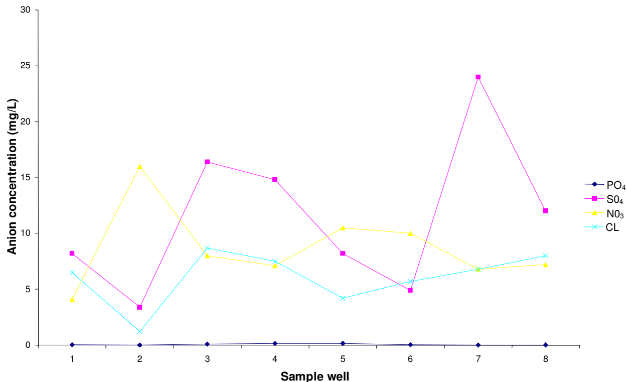
Figure 2. Distribution of anions in the groundwater samples.
