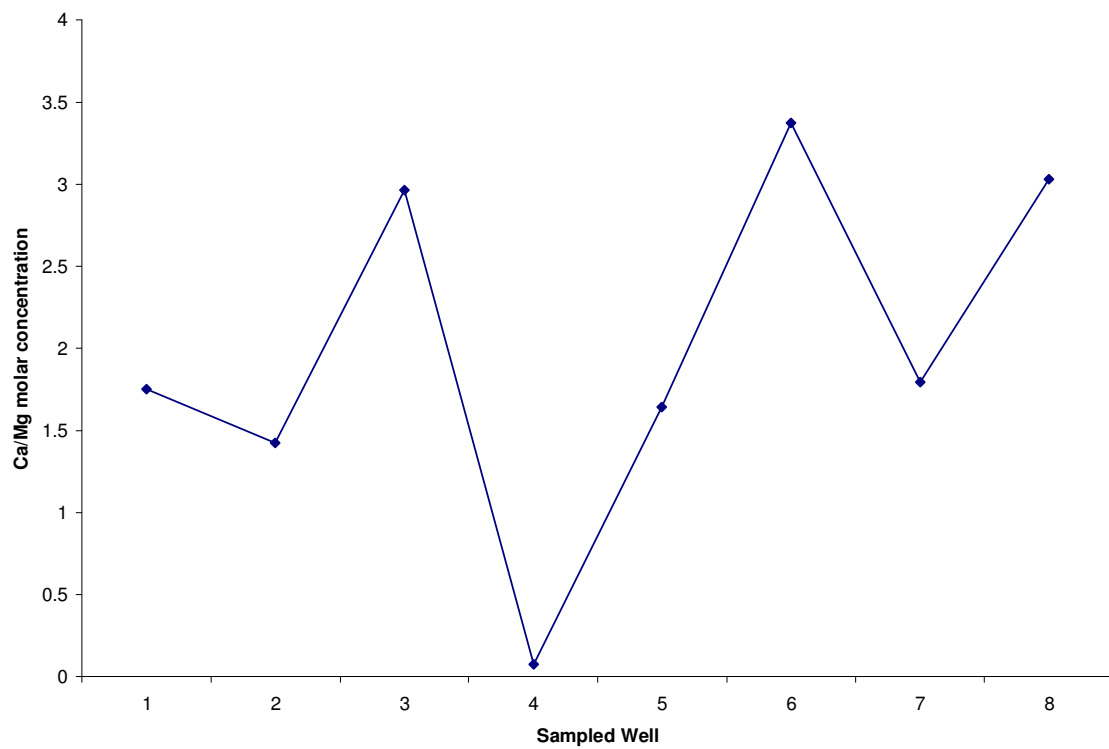
Figure 5. Plot of Ca/Mg molar ratio.
