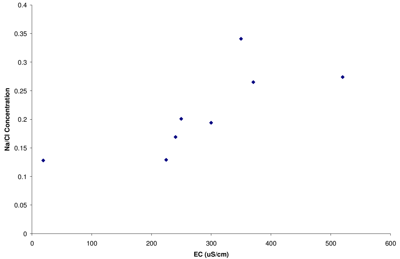
Figure 4. Plot of Na/Cl ratio vs EC.
