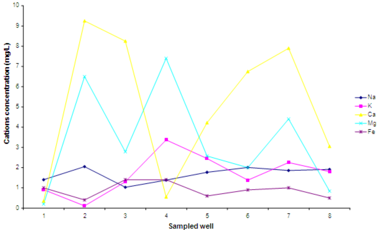
Figure 3. Distribution of cations in the groundwater samples.
