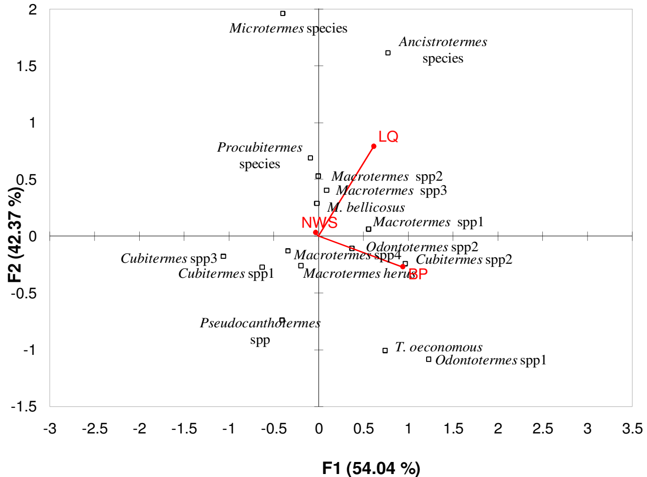
Figure 2. Ordination biplot based on canonical correspondence analysis of species/vegetation matrixes displaying 17.6% the inertia (= weighted variance) in species' abundances and 96% of variance in weighted averages with respect to the vegetation variables. The eigenvalues of axis 1 (horizontally) and axis 2 (vertically) are 0.29 and 0.23 respectively. The eigenvalue of axis 3 (not displayed) is 0.019.
