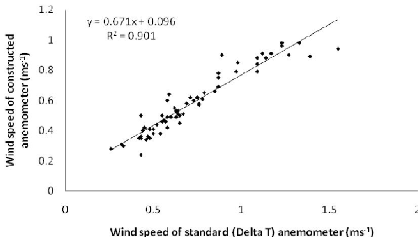
Figure 7. Calibration curve 1 showing the relationship between constructed and standard cup anemometer.
