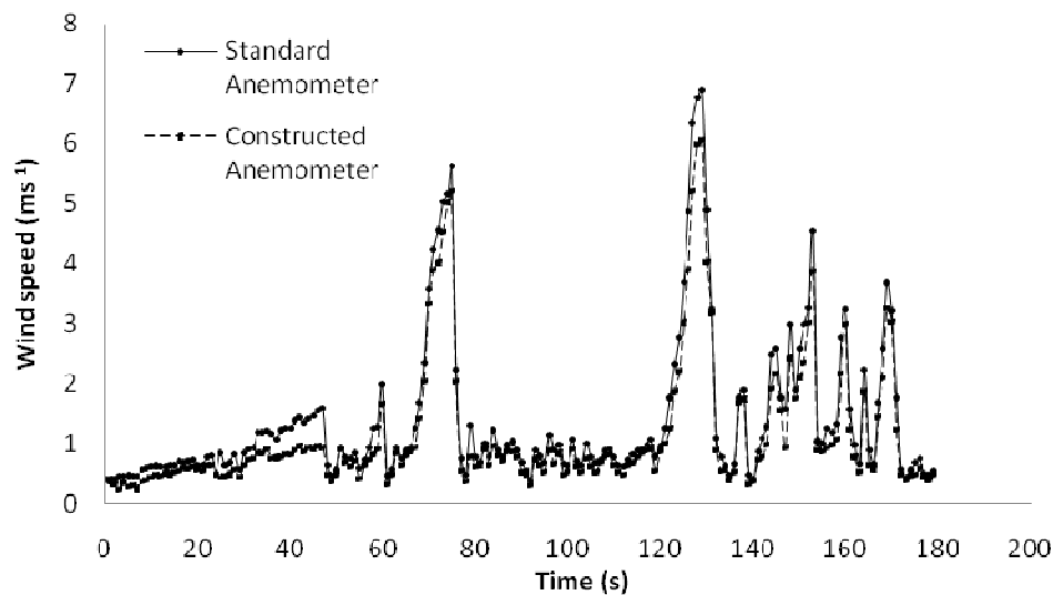
Figure 8. Wind speed measured from standard and constructed anemometer.
