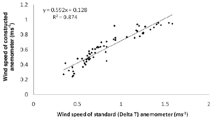
Figure 6. Calibration curve 1 showing the relationship between constructed and standard cup anemometer.
