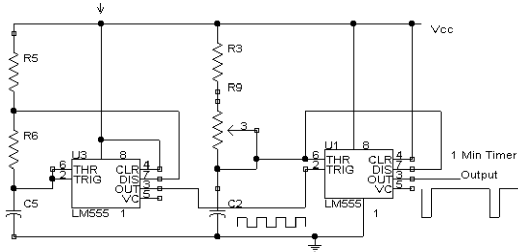
Figure 3. Pin connection of a stable clock and monostable 555 timer. When configured in a monostable mode, the 555 timer is so designed that, a pulse at the trigger input turns the timer on for a predetermined length of time.
