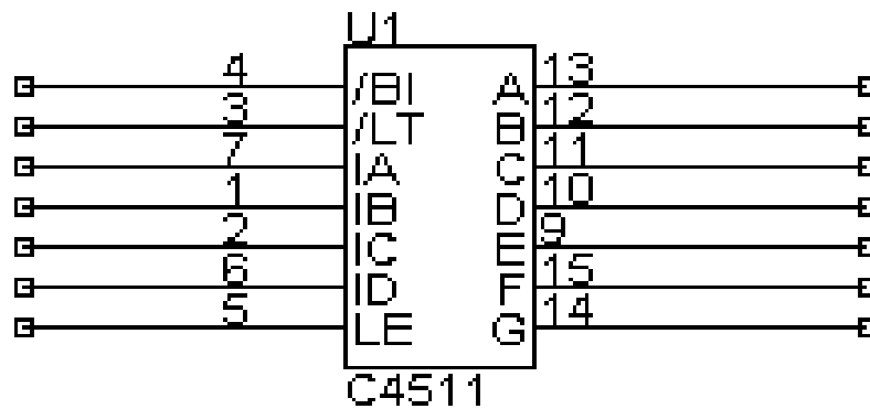
Figure 4. Pin configuration of 4511B latch/decoder.
