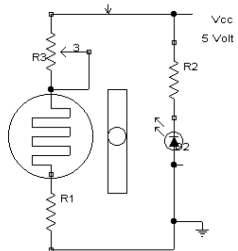
Figure 2. Schematic diagram of the input device.
