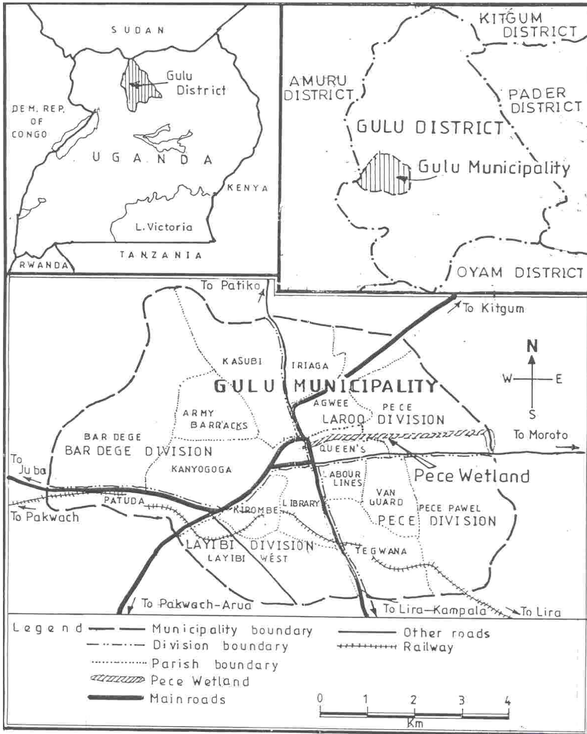
Figure 1. Location of Pece wetland in Gulu Municipality.
