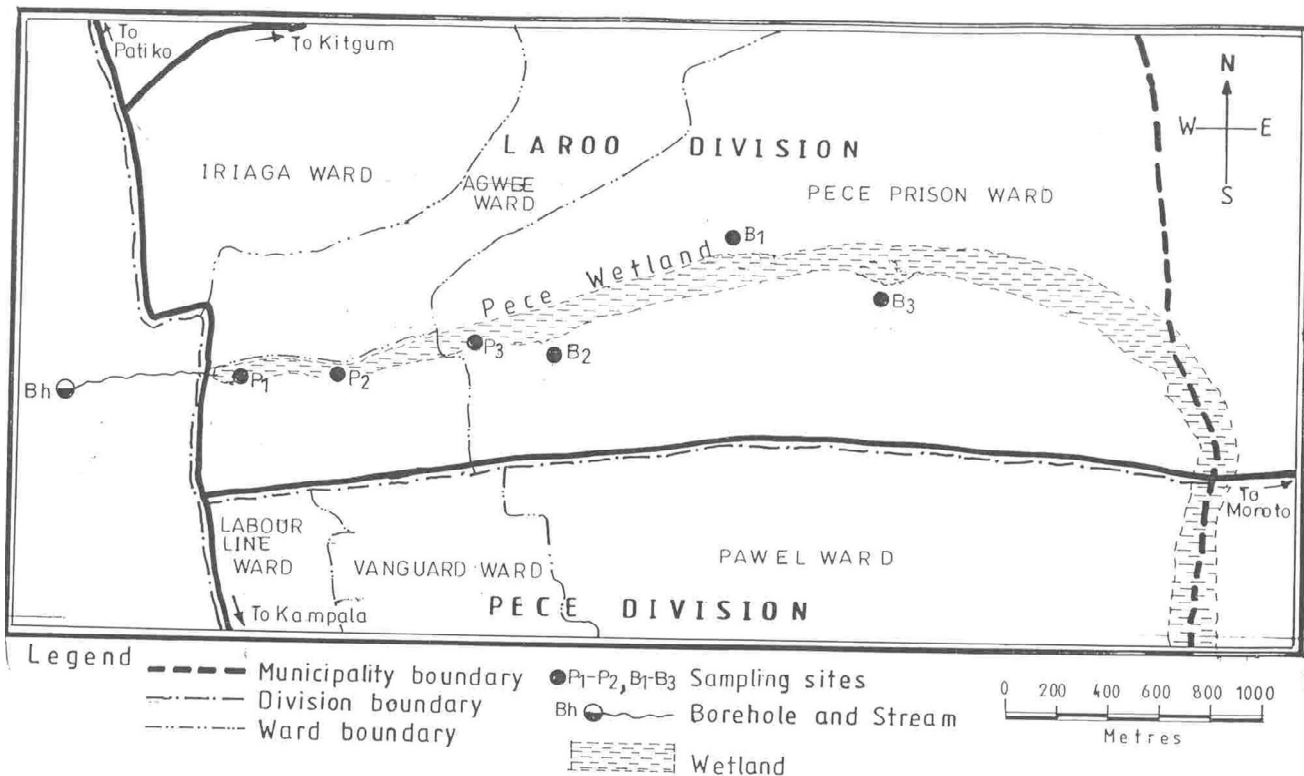
Figure 2. Location of water sources / sampling sites in Pece wetland.
