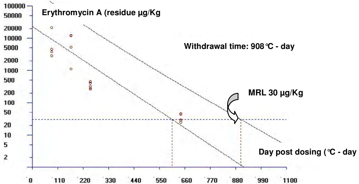
Figure 2. Linear regression line and upper one-sided tolerance limit (95%) linear regression line, with a confidence of 95%, of erythromycin concentrations in muscle tilapia treated with erythromycin for 7 days (50 mgkg -1 fish body weight.day -1 ) versus time. Degree-days are calculated by multiplying the mean daily water temperatures by the total number of days measured.
