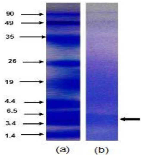
Figure 6. SDS-PAGE electrophoresis of the partially purified bacteriocin of B. megaterium 22. Lane a : Coomassie Brilliant blue-stained gel with small and large molecular weights of standard markers, lane b : Single band of partially-purified bacteriocin. Markers from top to bottom included: Bovine serum albumin ( E. coli ), ovalbumin (chicken egg), carbonic anhydrase (bovine erythrocytes), \beta -lactoglobulin (bovine milk), lysozyme (chicken egg white), \alpha -lactalbumin, aprotinin, insulin drain oxidized, and bacitracin. Sizes on the left are indicated in kDa.
