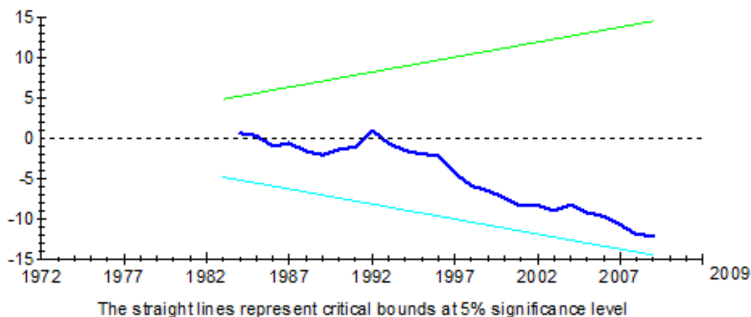
Figure 1. Plot of cumulative sum of recursive residuals.
